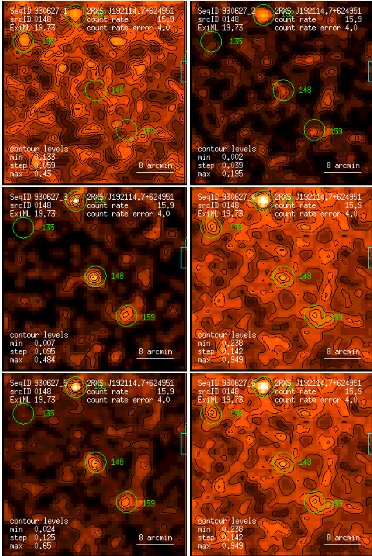
Figure 148: RASS 930627: detection 0148: band rate images, Gaussian filter: (1) PSPC channels 11 – 41, (2) 52 – 90, (3) 91 – 201, (4) 11 – 235, (5) 52 – 201, (6) 11 – 201. Broad band rates in counts/ks. Band rate contour levels in counts/ks/arcmin 2 .
