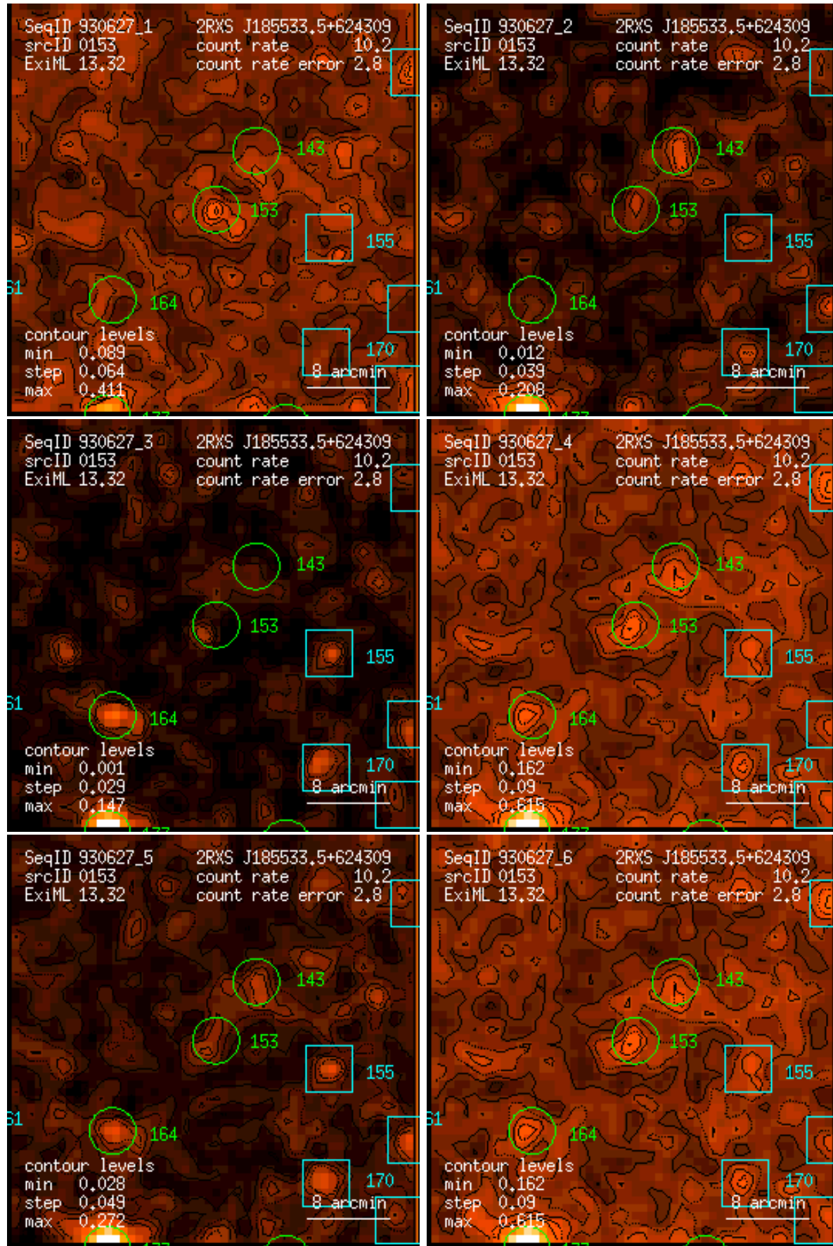
Figure 153: RASS 930627: detection 0153: band rate images, Gaussian filter: (1) PSPC channels 11 – 41, (2) 52 – 90, (3) 91 – 201, (4) 11 – 235, (5) 52 – 201, (6) 11 – 201. Broad band rates in counts/ks. Band rate contour levels in counts/ks/arcmin 2 .
