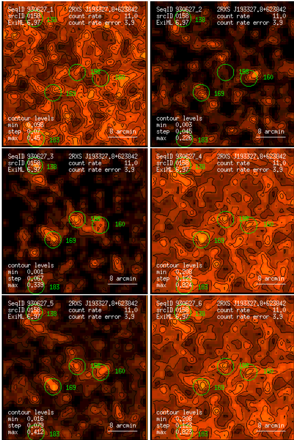
Figure 158: RASS 930627: detection 0158: band rate images, Gaussian filter: (1) PSPC channels 11 – 41, (2) 52 – 90, (3) 91 – 201, (4) 11 – 235, (5) 52 – 201, (6) 11 – 201. Broad band rates in counts/ks. Band rate contour levels in counts/ks/arcmin 2 .
