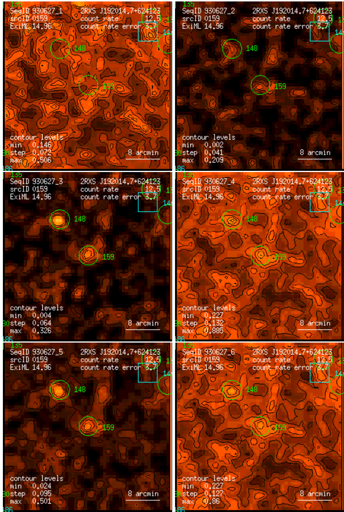
Figure 159: RASS 930627: detection 0159: band rate images, Gaussian filter: (1) PSPC channels 11 – 41, (2) 52 – 90, (3) 91 – 201, (4) 11 – 235, (5) 52 – 201, (6) 11 – 201. Broad band rates in counts/ks. Band rate contour levels in counts/ks/arcmin 2 .
