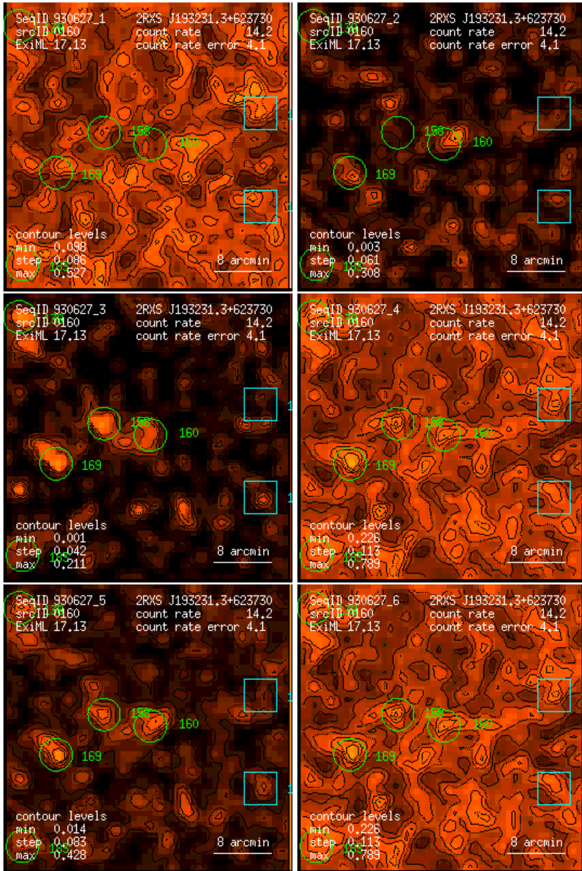
Figure 160: RASS 930627: detection 0160: band rate images, Gaussian filter: (1) PSPC channels 11 – 41, (2) 52 – 90, (3) 91 – 201, (4) 11 – 235, (5) 52 – 201, (6) 11 – 201. Broad band rates in counts/ks. Band rate contour levels in counts/ks/arcmin 2 .
