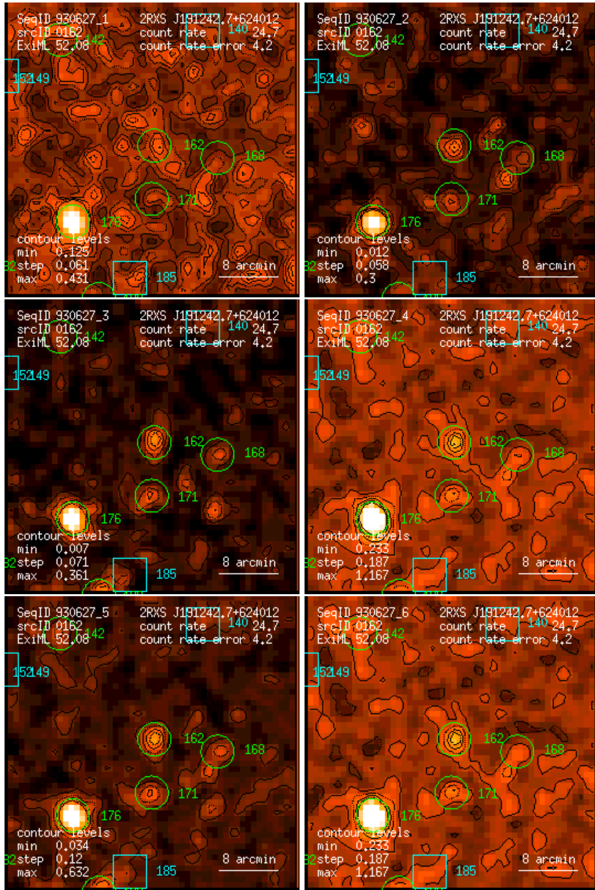
Figure 162: RASS 930627: detection 0162: band rate images, Gaussian filter: (1) PSPC channels 11 – 41, (2) 52 – 90, (3) 91 – 201, (4) 11 – 235, (5) 52 – 201, (6) 11 – 201. Broad band rates in counts/ks. Band rate contour levels in counts/ks/arcmin 2 .
