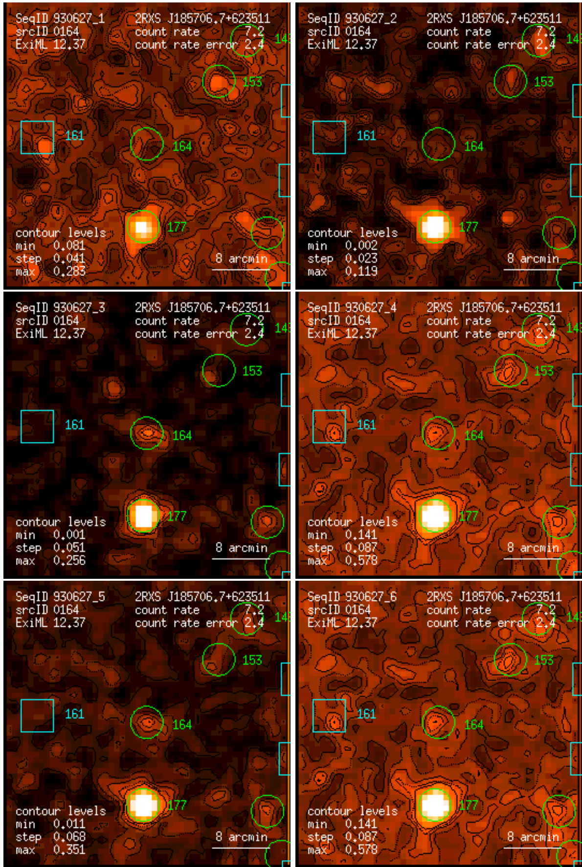
Figure 164: RASS 930627: detection 0164: band rate images, Gaussian filter: (1) PSPC channels 11 – 41, (2) 52 – 90, (3) 91 – 201, (4) 11 – 235, (5) 52 – 201, (6) 11 – 201. Broad band rates in counts/ks. Band rate contour levels in counts/ks/arcmin 2 .
