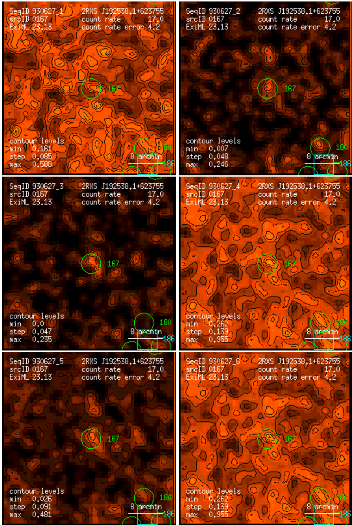
Figure 167: RASS 930627: detection 0167: band rate images, Gaussian filter: (1) PSPC channels 11 – 41, (2) 52 – 90, (3) 91 – 201, (4) 11 – 235, (5) 52 – 201, (6) 11 – 201. Broad band rates in counts/ks. Band rate contour levels in counts/ks/arcmin 2 .
