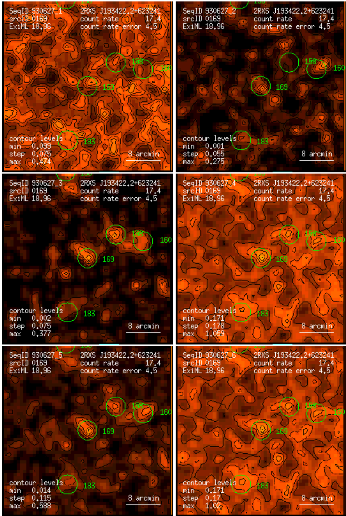
Figure 169: RASS 930627: detection 0169: band rate images, Gaussian filter: (1) PSPC channels 11 – 41, (2) 52 – 90, (3) 91 – 201, (4) 11 – 235, (5) 52 – 201, (6) 11 – 201. Broad band rates in counts/ks. Band rate contour levels in counts/ks/arcmin 2 .
