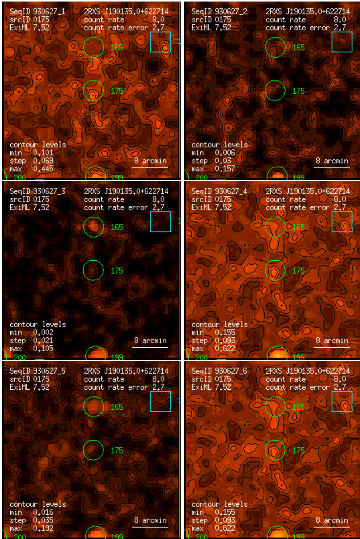
Figure 175: RASS 930627: detection 0175: band rate images, Gaussian filter: (1) PSPC channels 11 – 41, (2) 52 – 90, (3) 91 – 201, (4) 11 – 235, (5) 52 – 201, (6) 11 – 201. Broad band rates in counts/ks. Band rate contour levels in counts/ks/arcmin 2 .
