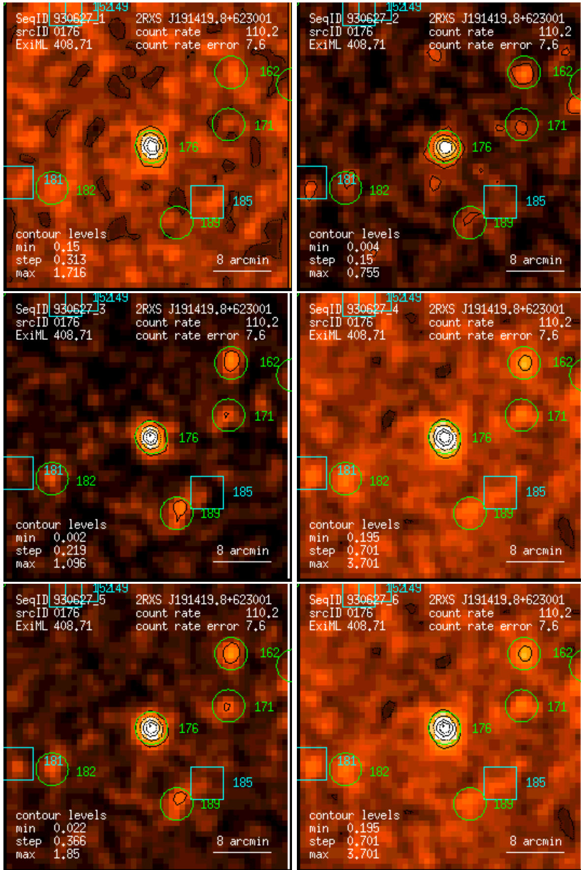
Figure 176: RASS 930627: detection 0176: band rate images, Gaussian filter: (1) PSPC channels 11 – 41, (2) 52 – 90, (3) 91 – 201, (4) 11 – 235, (5) 52 – 201, (6) 11 – 201. Broad band rates in counts/ks. Band rate contour levels in counts/ks/arcmin 2 .
