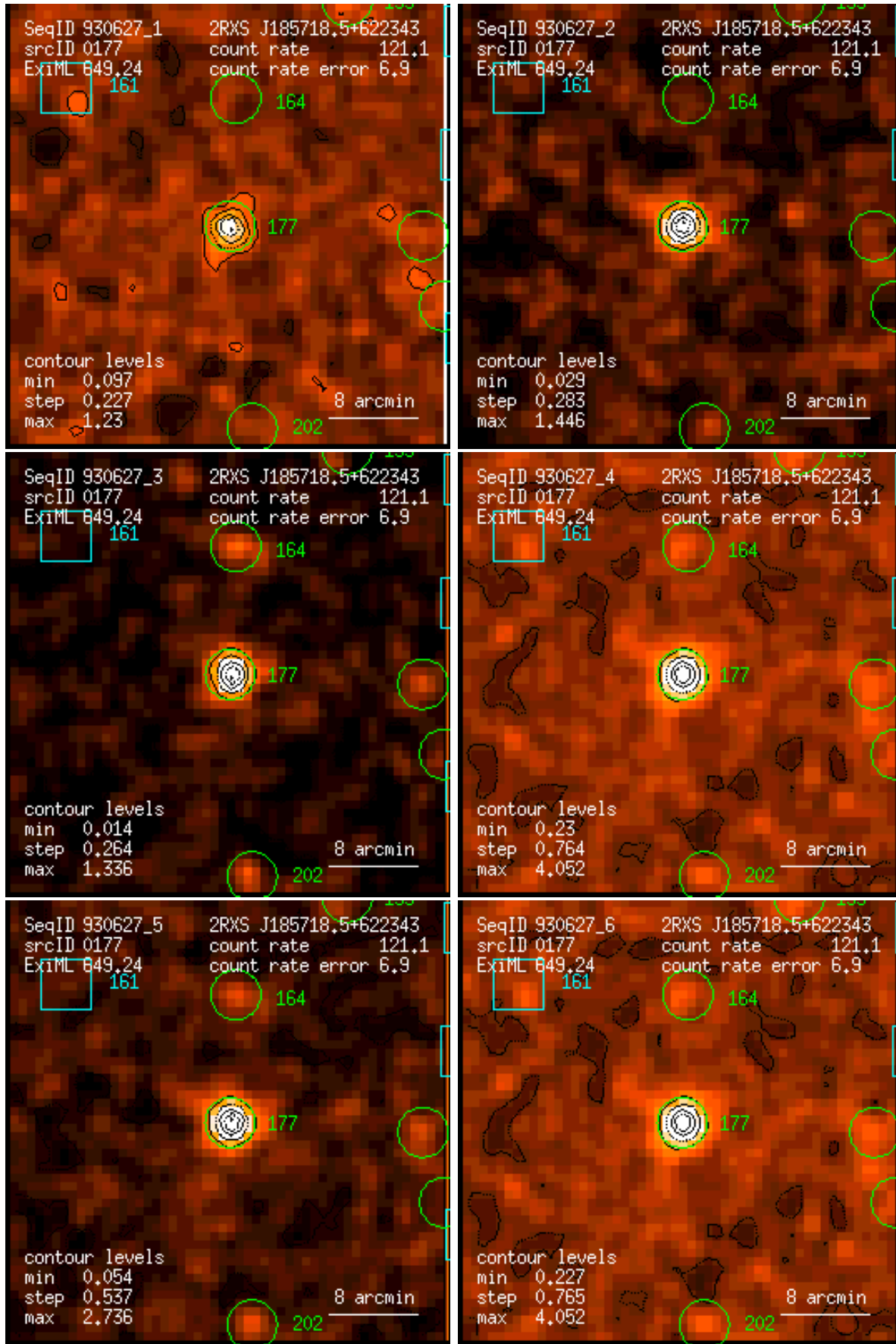
Figure 177: RASS 930627: detection 0177: band rate images, Gaussian filter: (1) PSPC channels 11 – 41, (2) 52 – 90, (3) 91 – 201, (4) 11 – 235, (5) 52 – 201, (6) 11 – 201. Broad band rates in counts/ks. Band rate contour levels in counts/ks/arcmin 2 .
