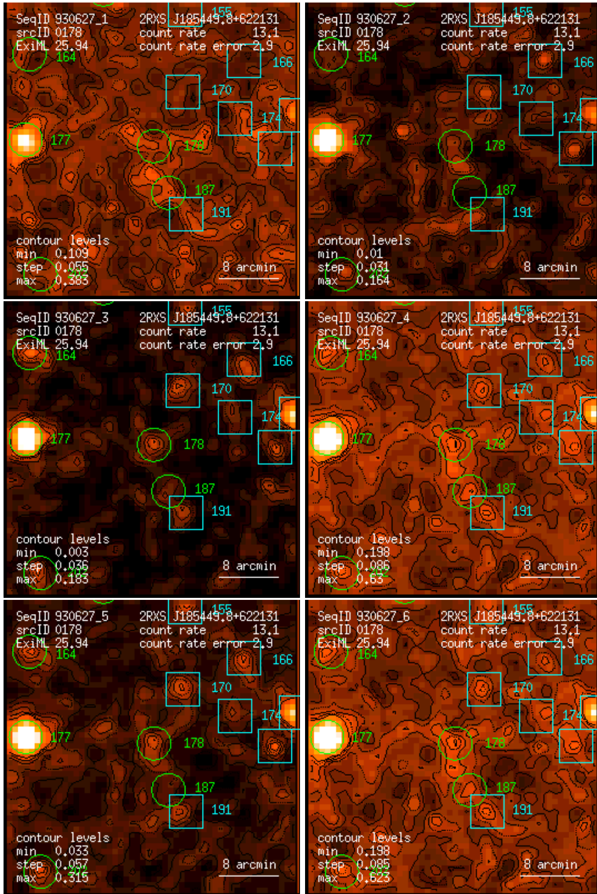
Figure 178: RASS 930627: detection 0178: band rate images, Gaussian filter: (1) PSPC channels 11 – 41, (2) 52 – 90, (3) 91 – 201, (4) 11 – 235, (5) 52 – 201, (6) 11 – 201. Broad band rates in counts/ks. Band rate contour levels in counts/ks/arcmin 2 .
