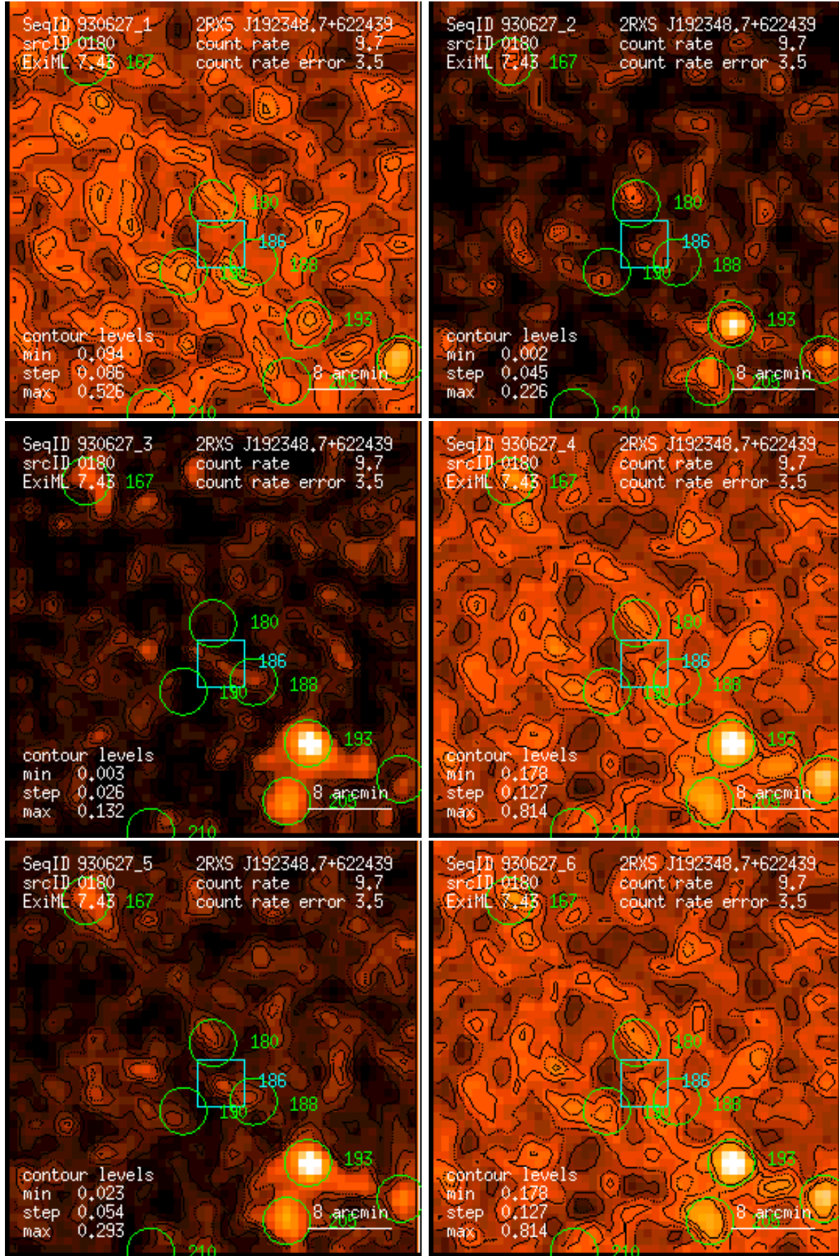
Figure 180: RASS 930627: detection 0180: band rate images, Gaussian filter: (1) PSPC channels 11 – 41, (2) 52 – 90, (3) 91 – 201, (4) 11 – 235, (5) 52 – 201, (6) 11 – 201. Broad band rates in counts/ks. Band rate contour levels in counts/ks/arcmin 2 .
