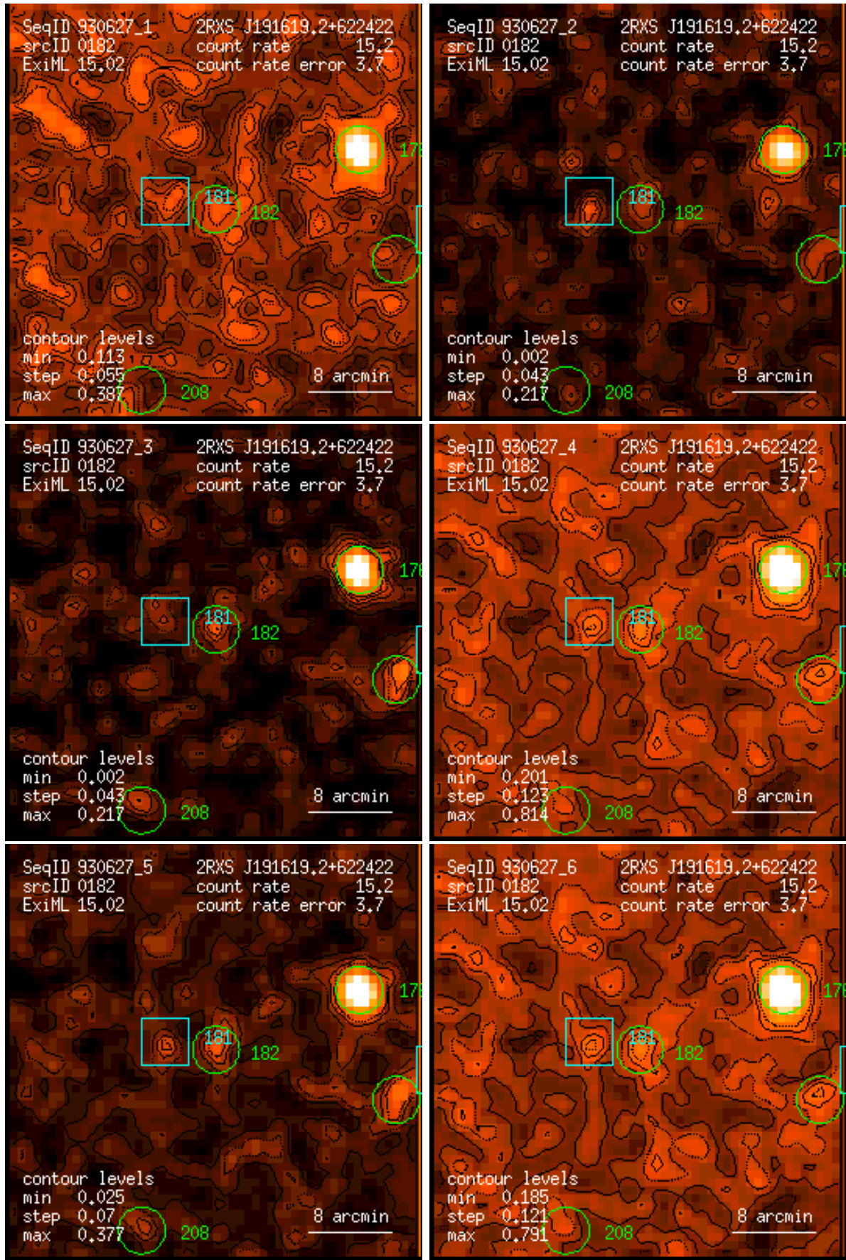
Figure 182: RASS 930627: detection 0182: band rate images, Gaussian filter: (1) PSPC channels 11 – 41, (2) 52 – 90, (3) 91 – 201, (4) 11 – 235, (5) 52 – 201, (6) 11 – 201. Broad band rates in counts/ks. Band rate contour levels in counts/ks/arcmin 2 .
