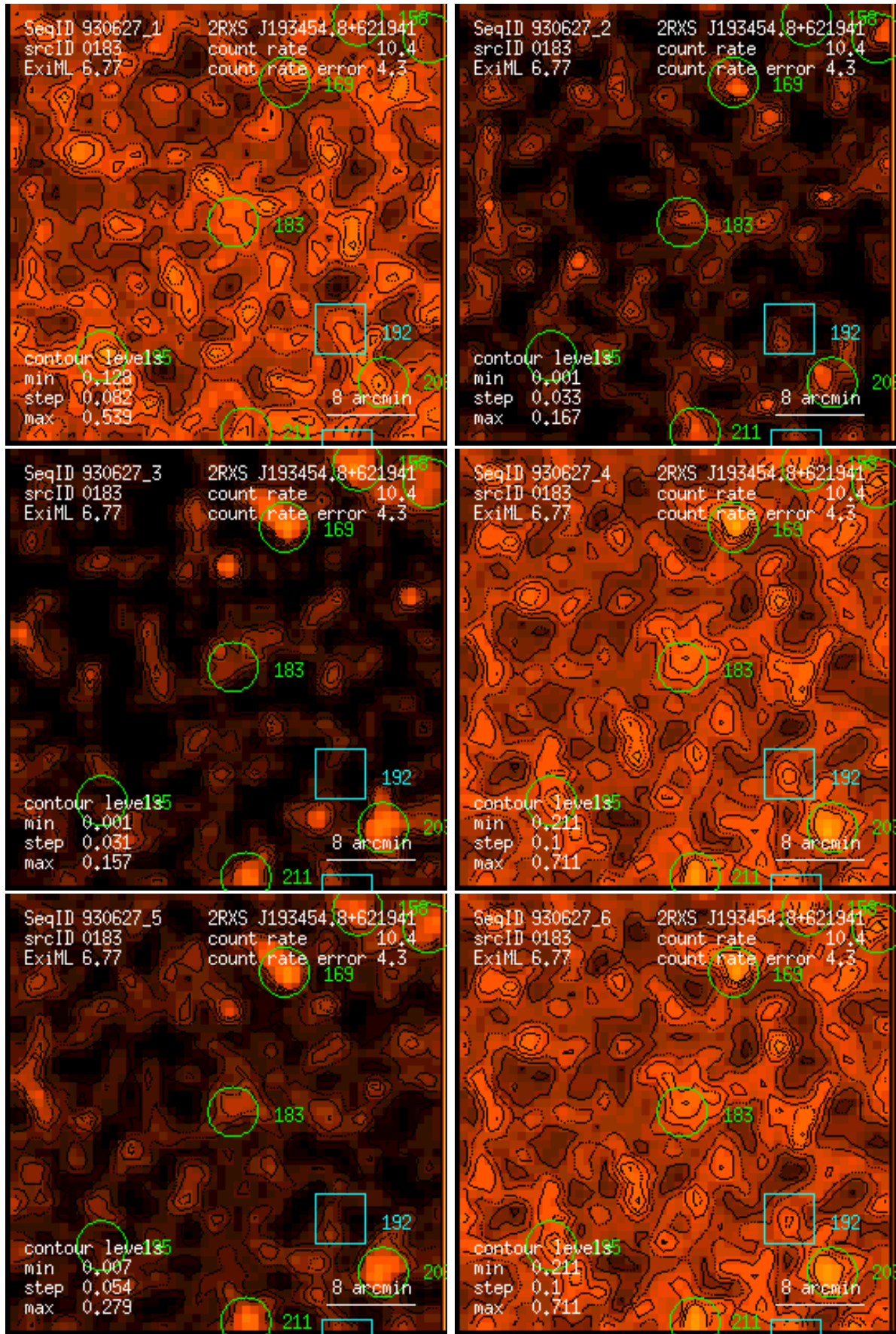
Figure 183: RASS 930627: detection 0183: band rate images, Gaussian filter: (1) PSPC channels 11 – 41, (2) 52 – 90, (3) 91 – 201, (4) 11 – 235, (5) 52 – 201, (6) 11 – 201. Broad band rates in counts/ks. Band rate contour levels in counts/ks/arcmin 2 .
