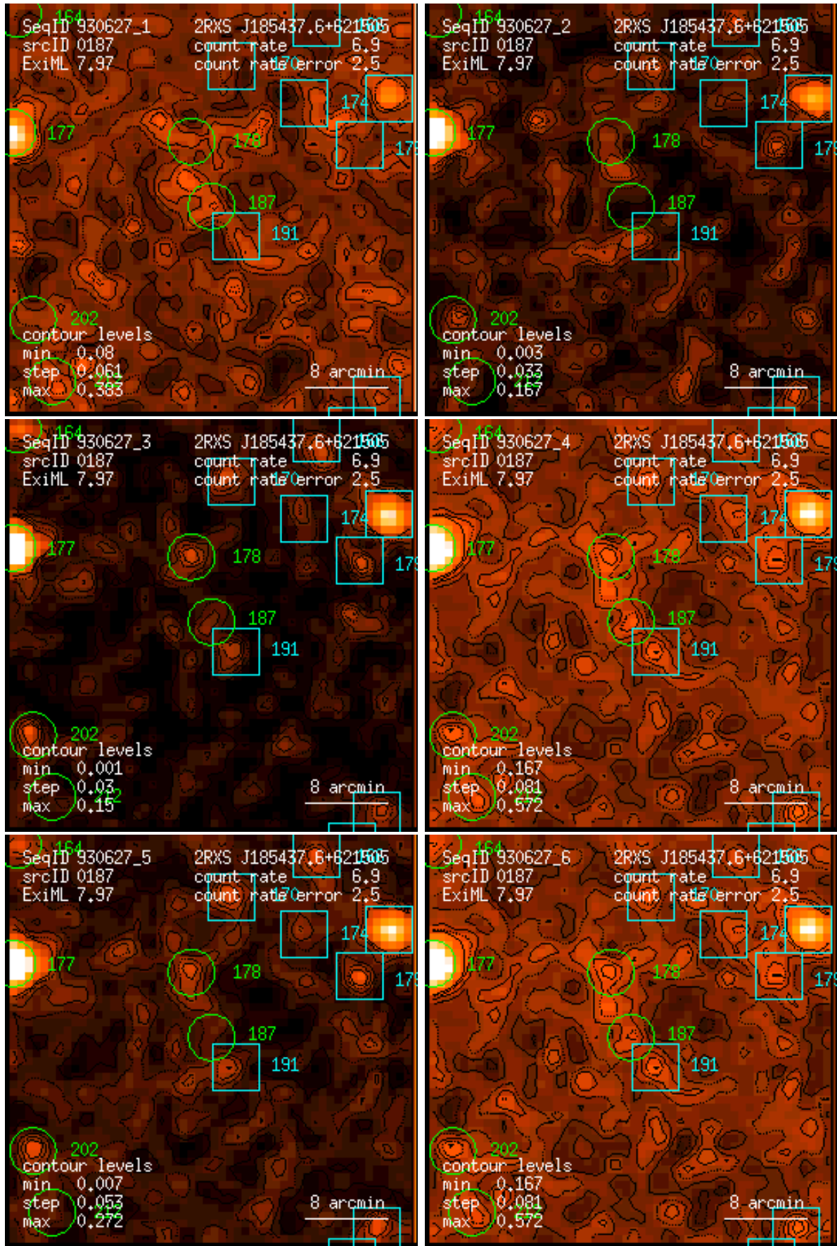
Figure 187: RASS 930627: detection 0187: band rate images, Gaussian filter: (1) PSPC channels 11 – 41, (2) 52 – 90, (3) 91 – 201, (4) 11 – 235, (5) 52 – 201, (6) 11 – 201. Broad band rates in counts/ks. Band rate contour levels in counts/ks/arcmin 2 .
