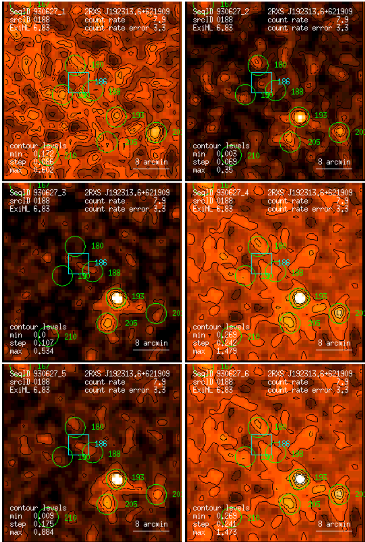
Figure 188: RASS 930627: detection 0188: band rate images, Gaussian filter: (1) PSPC channels 11 – 41, (2) 52 – 90, (3) 91 – 201, (4) 11 – 235, (5) 52 – 201, (6) 11 – 201. Broad band rates in counts/ks. Band rate contour levels in counts/ks/arcmin 2 .
