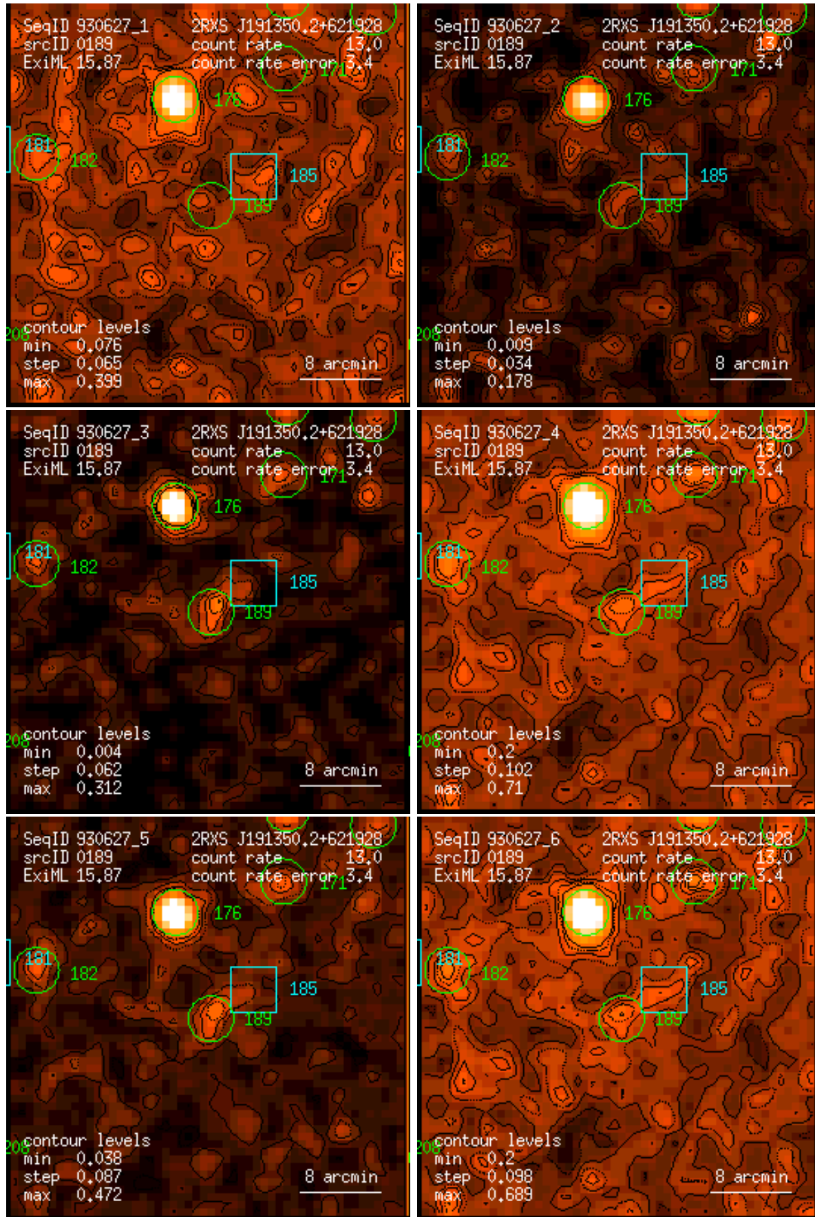
Figure 189: RASS 930627: detection 0189: band rate images, Gaussian filter: (1) PSPC channels 11 – 41, (2) 52 – 90, (3) 91 – 201, (4) 11 – 235, (5) 52 – 201, (6) 11 – 201. Broad band rates in counts/ks. Band rate contour levels in counts/ks/arcmin 2 .
