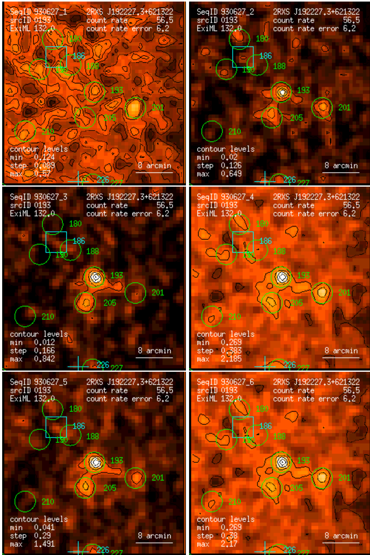
Figure 193: RASS 930627: detection 0193: band rate images, Gaussian filter: (1) PSPC channels 11 – 41, (2) 52 – 90, (3) 91 – 201, (4) 11 – 235, (5) 52 – 201, (6) 11 – 201. Broad band rates in counts/ks. Band rate contour levels in counts/ks/arcmin 2 .
