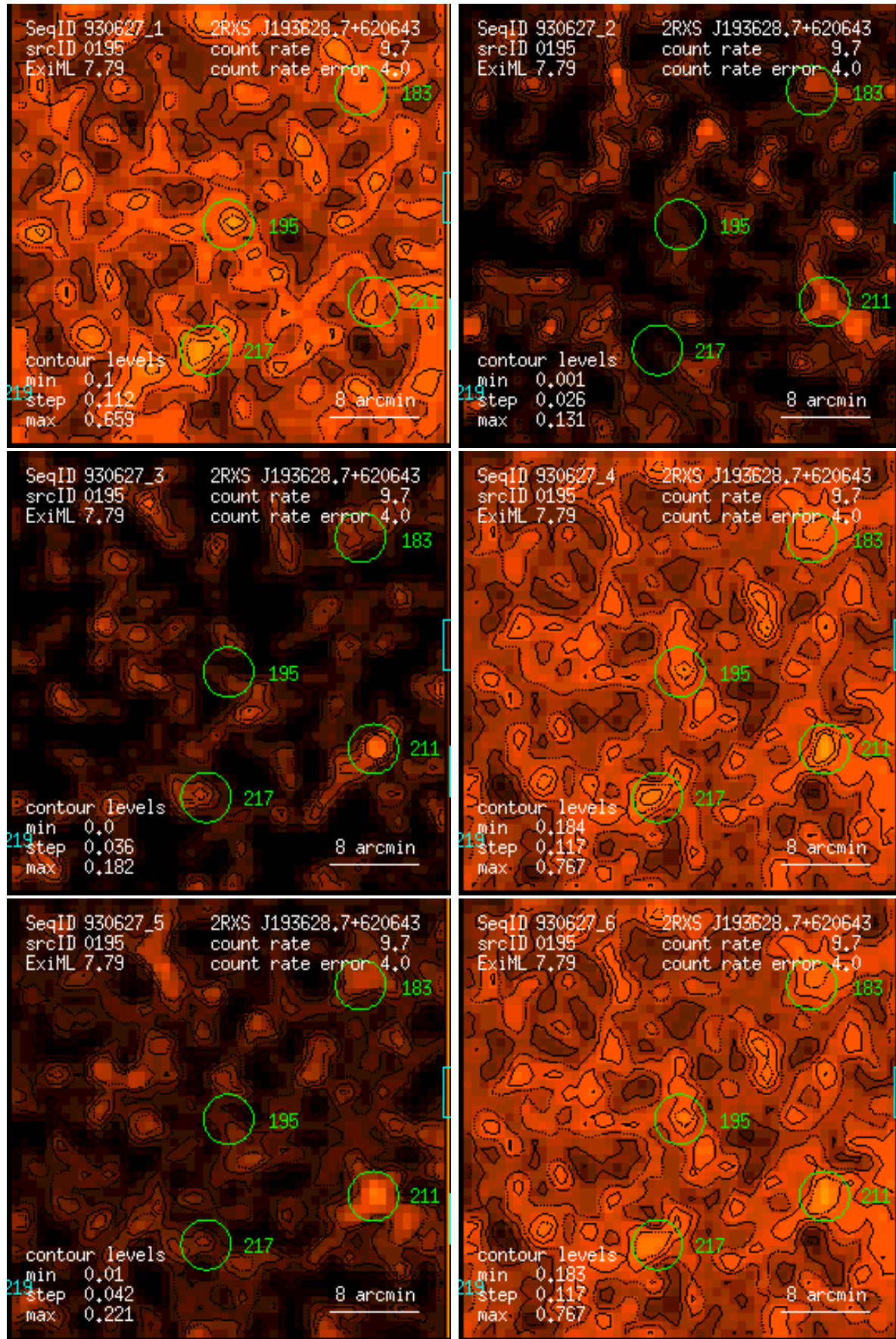
Figure 195: RASS 930627: detection 0195: band rate images, Gaussian filter: (1) PSPC channels 11 – 41, (2) 52 – 90, (3) 91 – 201, (4) 11 – 235, (5) 52 – 201, (6) 11 – 201. Broad band rates in counts/ks. Band rate contour levels in counts/ks/arcmin 2 .
