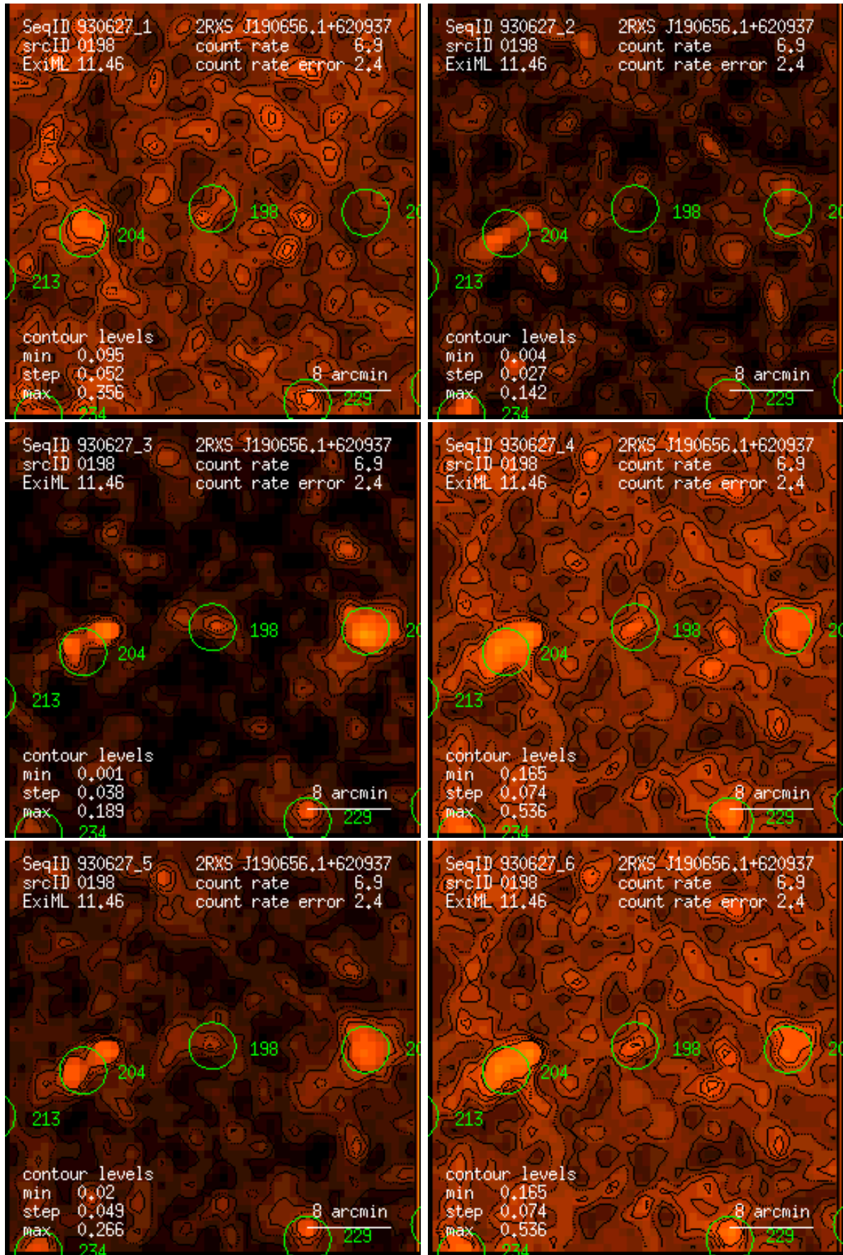
Figure 198: RASS 930627: detection 0198: band rate images, Gaussian filter: (1) PSPC channels 11 – 41, (2) 52 – 90, (3) 91 – 201, (4) 11 – 235, (5) 52 – 201, (6) 11 – 201. Broad band rates in counts/ks. Band rate contour levels in counts/ks/arcmin 2 .
