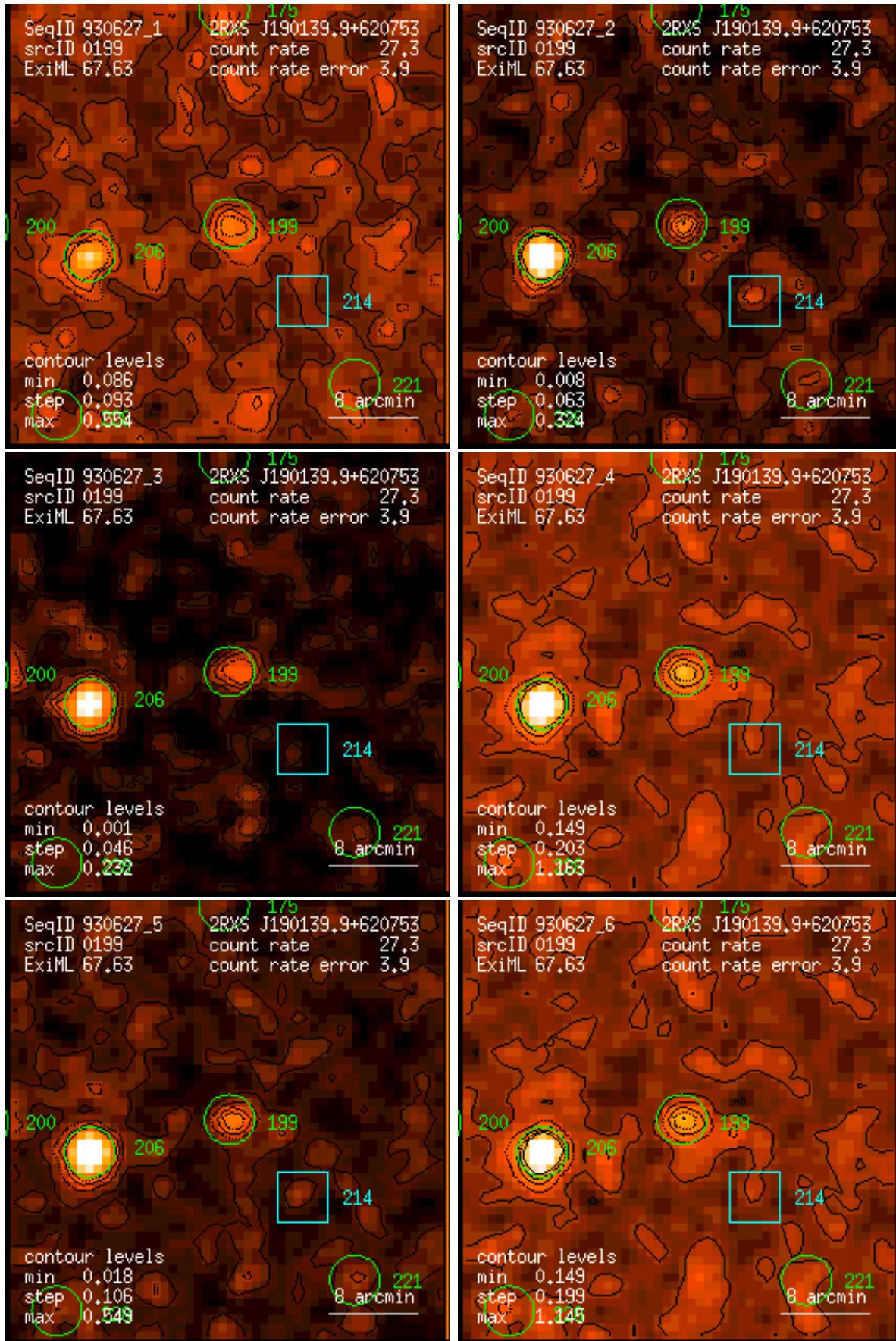
Figure 199: RASS 930627: detection 0199: band rate images, Gaussian filter: (1) PSPC channels 11 – 41, (2) 52 – 90, (3) 91 – 201, (4) 11 – 235, (5) 52 – 201, (6) 11 – 201. Broad band rates in counts/ks. Band rate contour levels in counts/ks/arcmin 2 .
