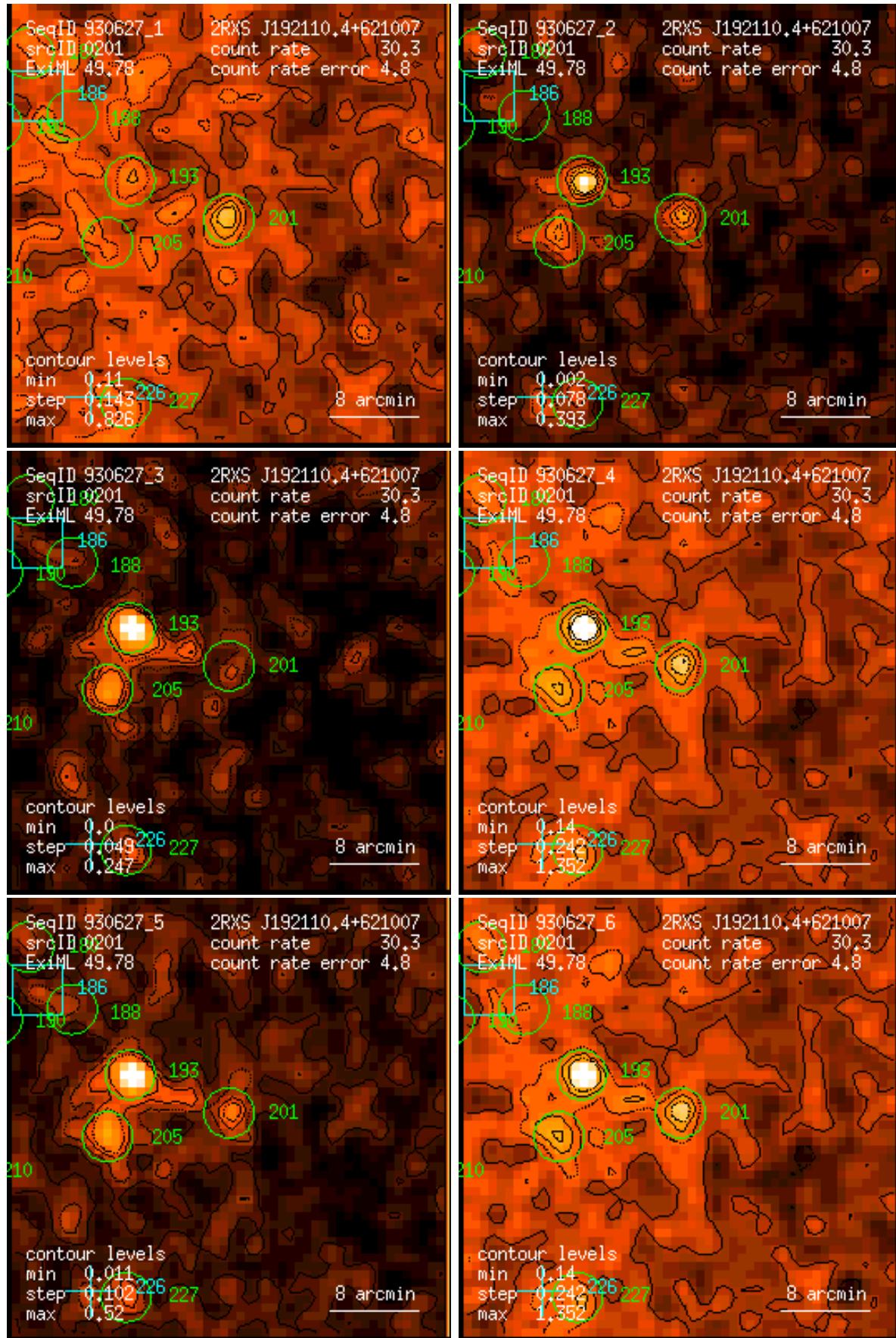
Figure 201: RASS 930627: detection 0201: band rate images, Gaussian filter: (1) PSPC channels 11 – 41, (2) 52 – 90, (3) 91 – 201, (4) 11 – 235, (5) 52 – 201, (6) 11 – 201. Broad band rates in counts/ks. Band rate contour levels in counts/ks/arcmin 2 .
