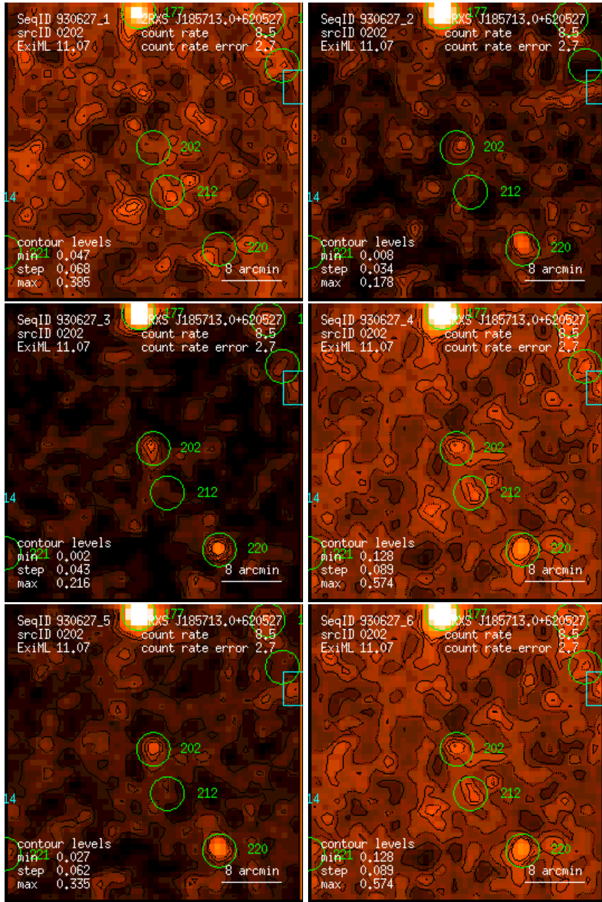
Figure 202: RASS 930627: detection 0202: band rate images, Gaussian filter: (1) PSPC channels 11 – 41, (2) 52 – 90, (3) 91 – 201, (4) 11 – 235, (5) 52 – 201, (6) 11 – 201. Broad band rates in counts/ks. Band rate contour levels in counts/ks/arcmin 2 .
