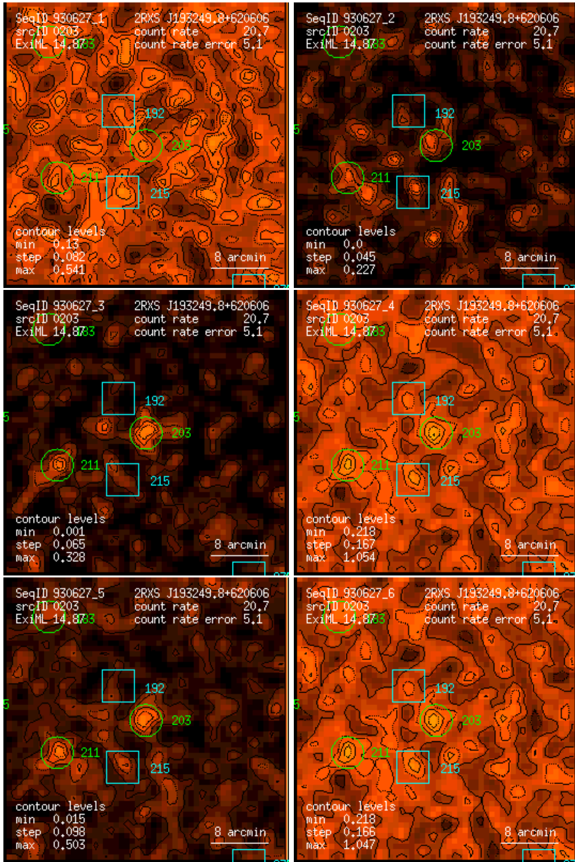
Figure 203: RASS 930627: detection 0203: band rate images, Gaussian filter: (1) PSPC channels 11 – 41, (2) 52 – 90, (3) 91 – 201, (4) 11 – 235, (5) 52 – 201, (6) 11 – 201. Broad band rates in counts/ks. Band rate contour levels in counts/ks/arcmin 2 .
