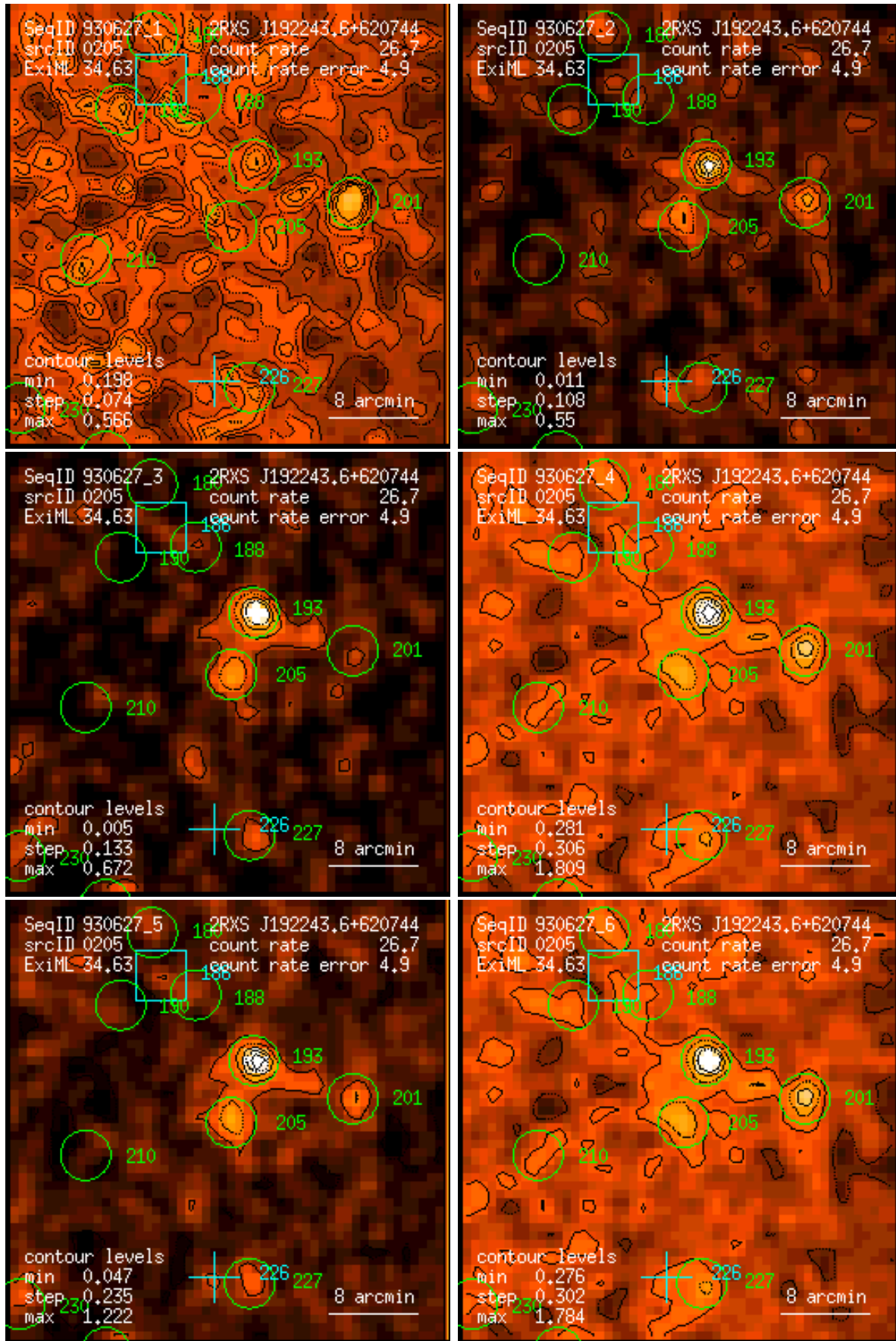
Figure 205: RASS 930627: detection 0205: band rate images, Gaussian filter: (1) PSPC channels 11 – 41, (2) 52 – 90, (3) 91 – 201, (4) 11 – 235, (5) 52 – 201, (6) 11 – 201. Broad band rates in counts/ks. Band rate contour levels in counts/ks/arcmin 2 .
