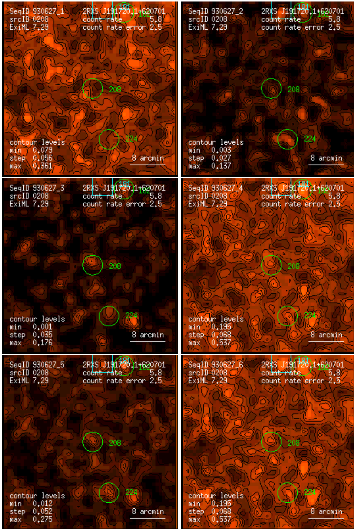
Figure 208: RASS 930627: detection 0208: band rate images, Gaussian filter: (1) PSPC channels 11 – 41, (2) 52 – 90, (3) 91 – 201, (4) 11 – 235, (5) 52 – 201, (6) 11 – 201. Broad band rates in counts/ks. Band rate contour levels in counts/ks/arcmin 2 .
