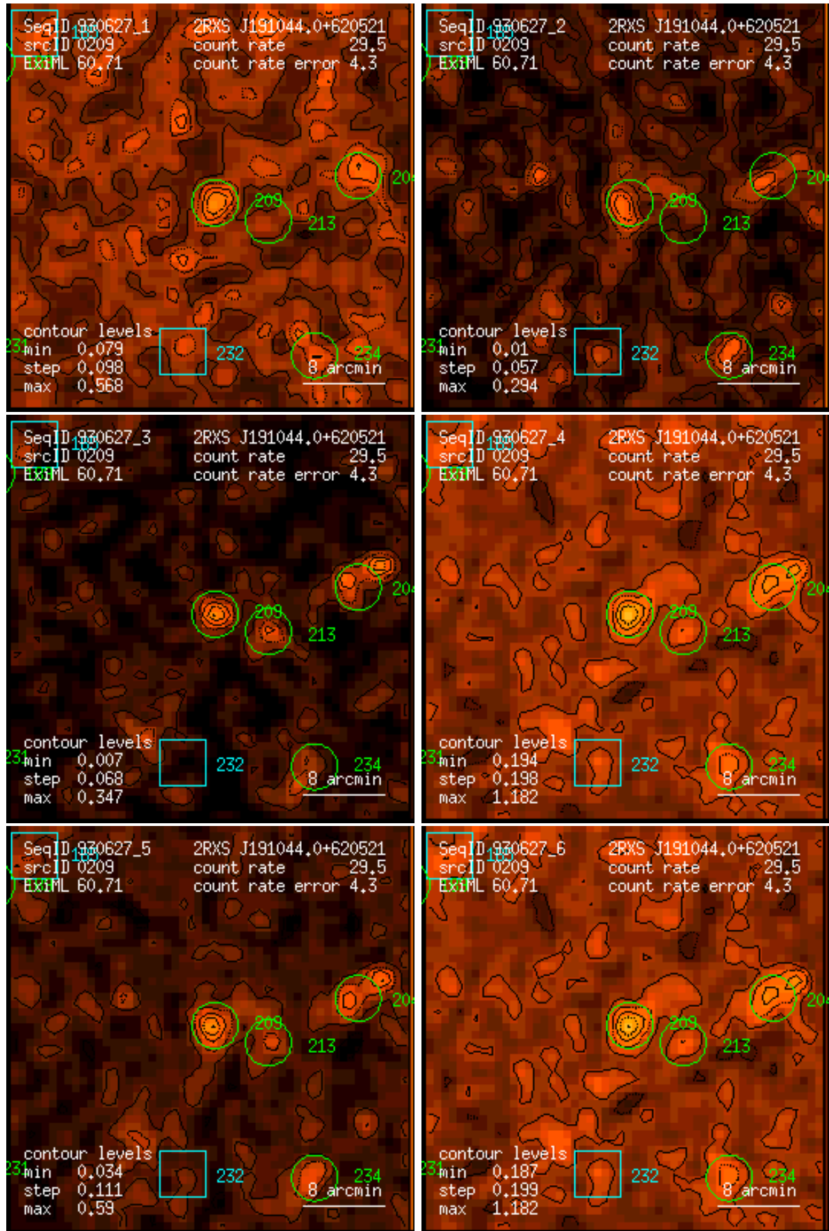
Figure 209: RASS 930627: detection 0209: band rate images, Gaussian filter: (1) PSPC channels 11 – 41, (2) 52 – 90, (3) 91 – 201, (4) 11 – 235, (5) 52 – 201, (6) 11 – 201. Broad band rates in counts/ks. Band rate contour levels in counts/ks/arcmin 2 .
