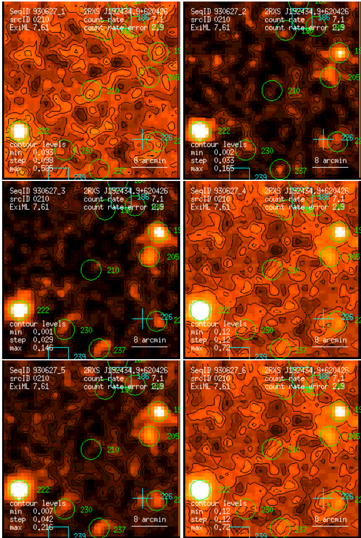
Figure 210: RASS 930627: detection 0210: band rate images, Gaussian filter: (1) PSPC channels 11 – 41, (2) 52 – 90, (3) 91 – 201, (4) 11 – 235, (5) 52 – 201, (6) 11 – 201. Broad band rates in counts/ks. Band rate contour levels in counts/ks/arcmin 2 .
