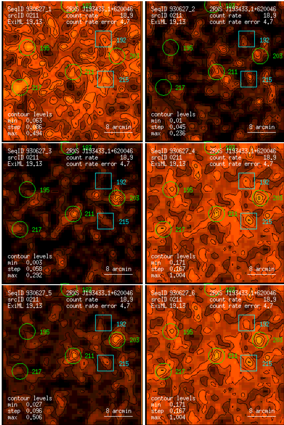
Figure 211: RASS 930627: detection 0211: band rate images, Gaussian filter: (1) PSPC channels 11 – 41, (2) 52 – 90, (3) 91 – 201, (4) 11 – 235, (5) 52 – 201, (6) 11 – 201. Broad band rates in counts/ks. Band rate contour levels in counts/ks/arcmin 2 .
