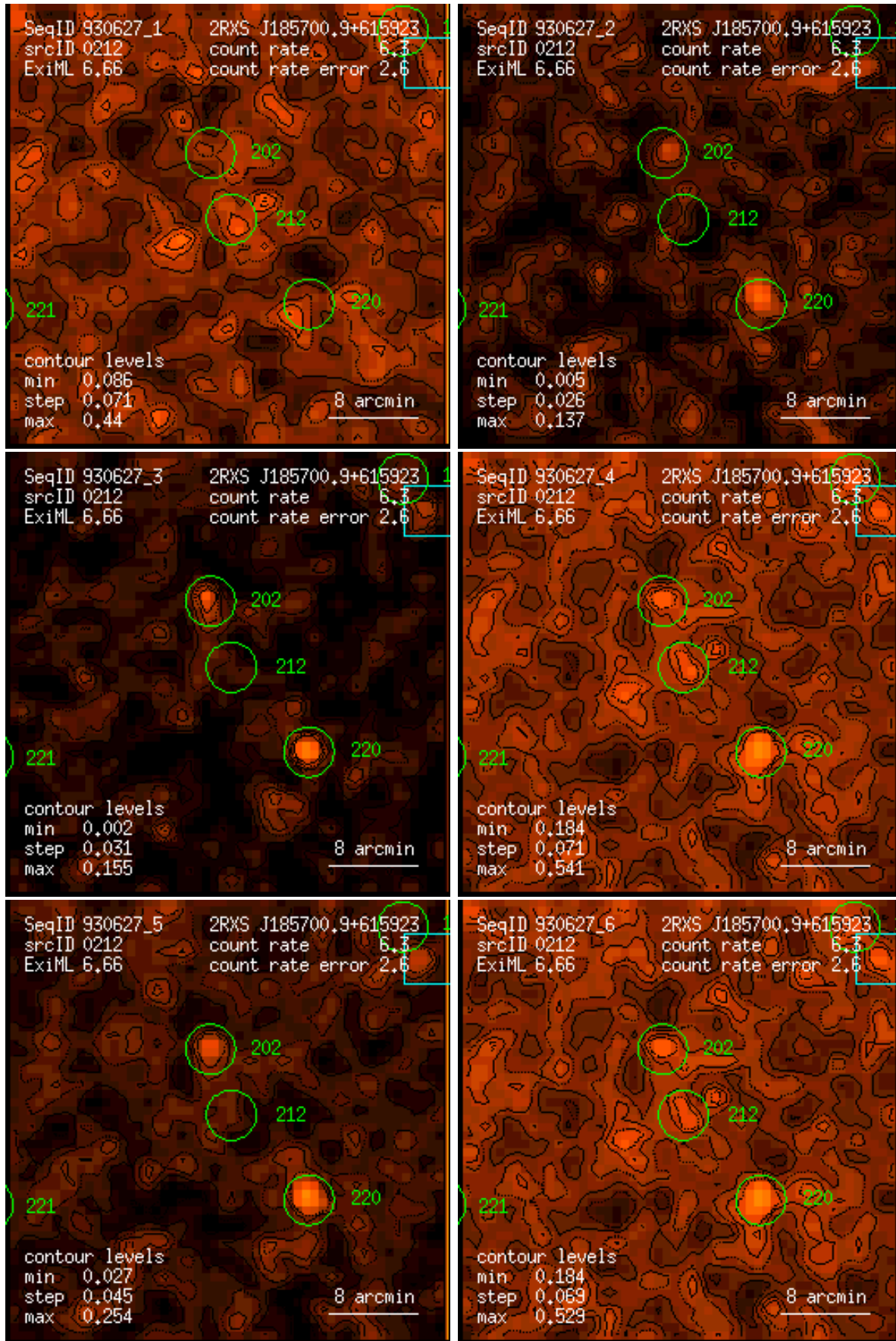
Figure 212: RASS 930627: detection 0212: band rate images, Gaussian filter: (1) PSPC channels 11 – 41, (2) 52 – 90, (3) 91 – 201, (4) 11 – 235, (5) 52 – 201, (6) 11 – 201. Broad band rates in counts/ks. Band rate contour levels in counts/ks/arcmin 2 .
