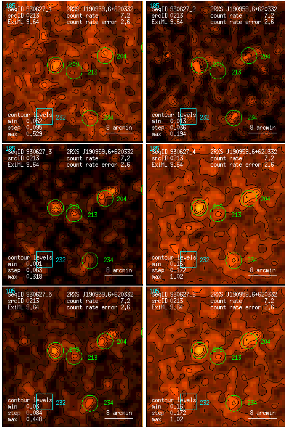
Figure 213: RASS 930627: detection 0213: band rate images, Gaussian filter: (1) PSPC channels 11 – 41, (2) 52 – 90, (3) 91 – 201, (4) 11 – 235, (5) 52 – 201, (6) 11 – 201. Broad band rates in counts/ks. Band rate contour levels in counts/ks/arcmin 2 .
