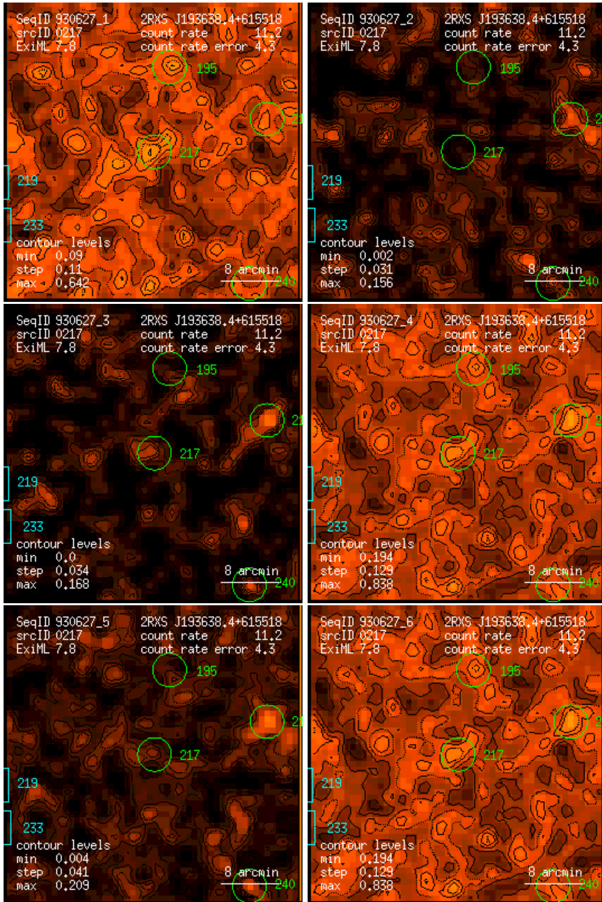
Figure 217: RASS 930627: detection 0217: band rate images, Gaussian filter: (1) PSPC channels 11 – 41, (2) 52 – 90, (3) 91 – 201, (4) 11 – 235, (5) 52 – 201, (6) 11 – 201. Broad band rates in counts/ks. Band rate contour levels in counts/ks/arcmin 2 .
