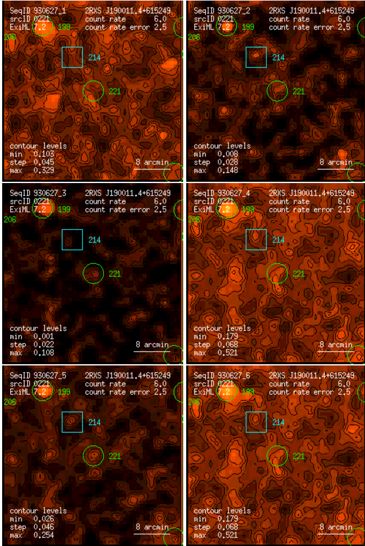
Figure 221: RASS 930627: detection 0221: band rate images, Gaussian filter: (1) PSPC channels 11 – 41, (2) 52 – 90, (3) 91 – 201, (4) 11 – 235, (5) 52 – 201, (6) 11 – 201. Broad band rates in counts/ks. Band rate contour levels in counts/ks/arcmin 2 .
