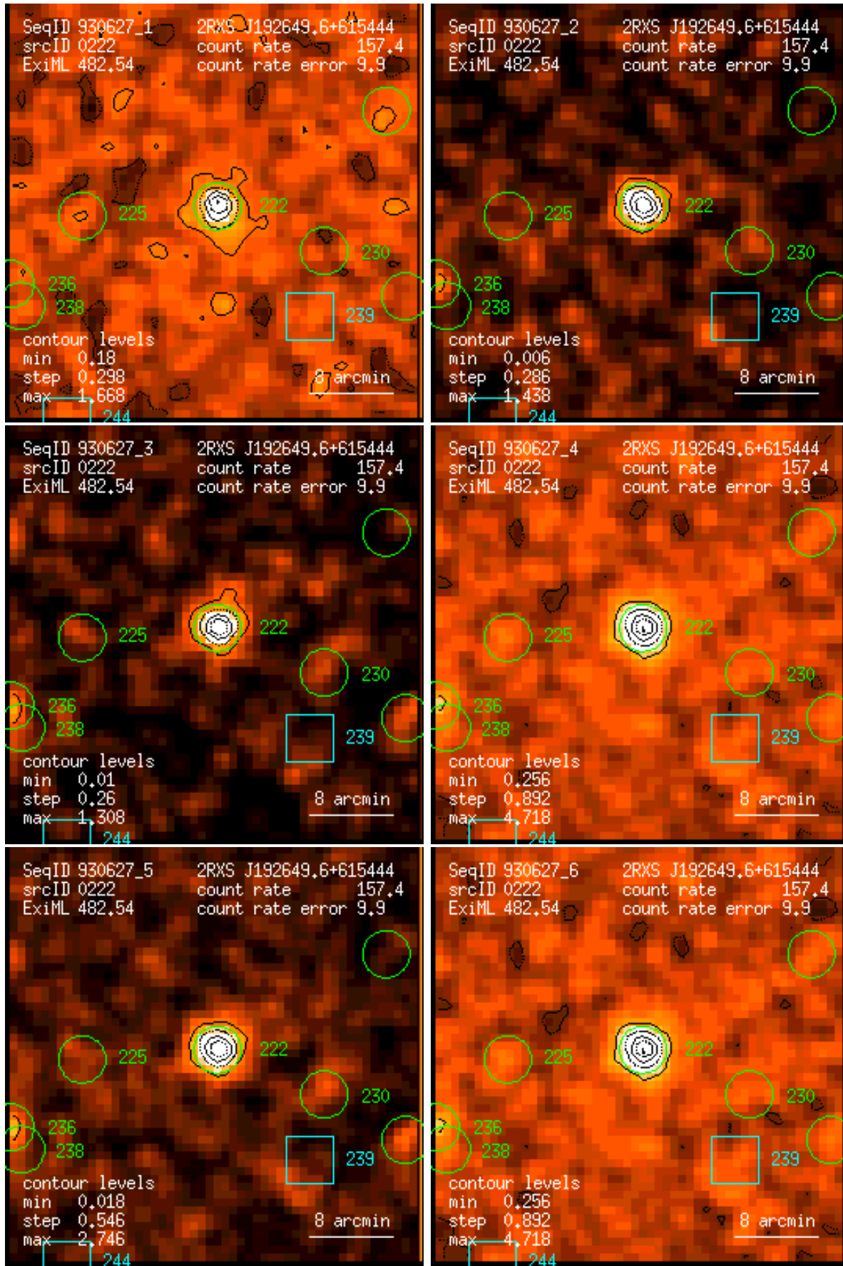
Figure 222: RASS 930627: detection 0222: band rate images, Gaussian filter: (1) PSPC channels 11 – 41, (2) 52 – 90, (3) 91 – 201, (4) 11 – 235, (5) 52 – 201, (6) 11 – 201. Broad band rates in counts/ks. Band rate contour levels in counts/ks/arcmin 2 .
