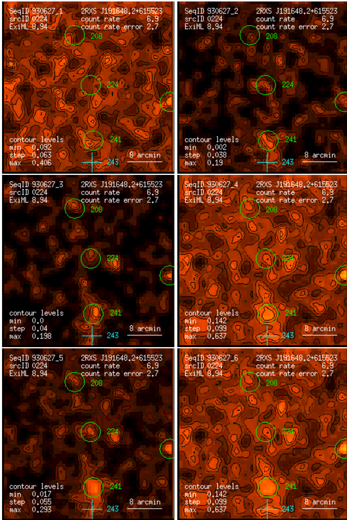
Figure 224: RASS 930627: detection 0224: band rate images, Gaussian filter: (1) PSPC channels 11 – 41, (2) 52 – 90, (3) 91 – 201, (4) 11 – 235, (5) 52 – 201, (6) 11 – 201. Broad band rates in counts/ks. Band rate contour levels in counts/ks/arcmin 2 .
