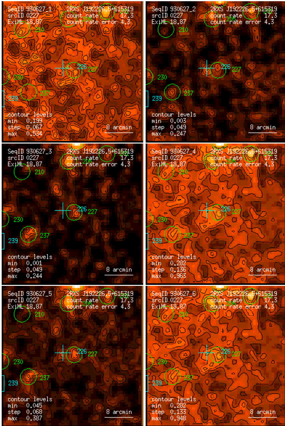
Figure 227: RASS 930627: detection 0227: band rate images, Gaussian filter: (1) PSPC channels 11 – 41, (2) 52 – 90, (3) 91 – 201, (4) 11 – 235, (5) 52 – 201, (6) 11 – 201. Broad band rates in counts/ks. Band rate contour levels in counts/ks/arcmin 2 .
