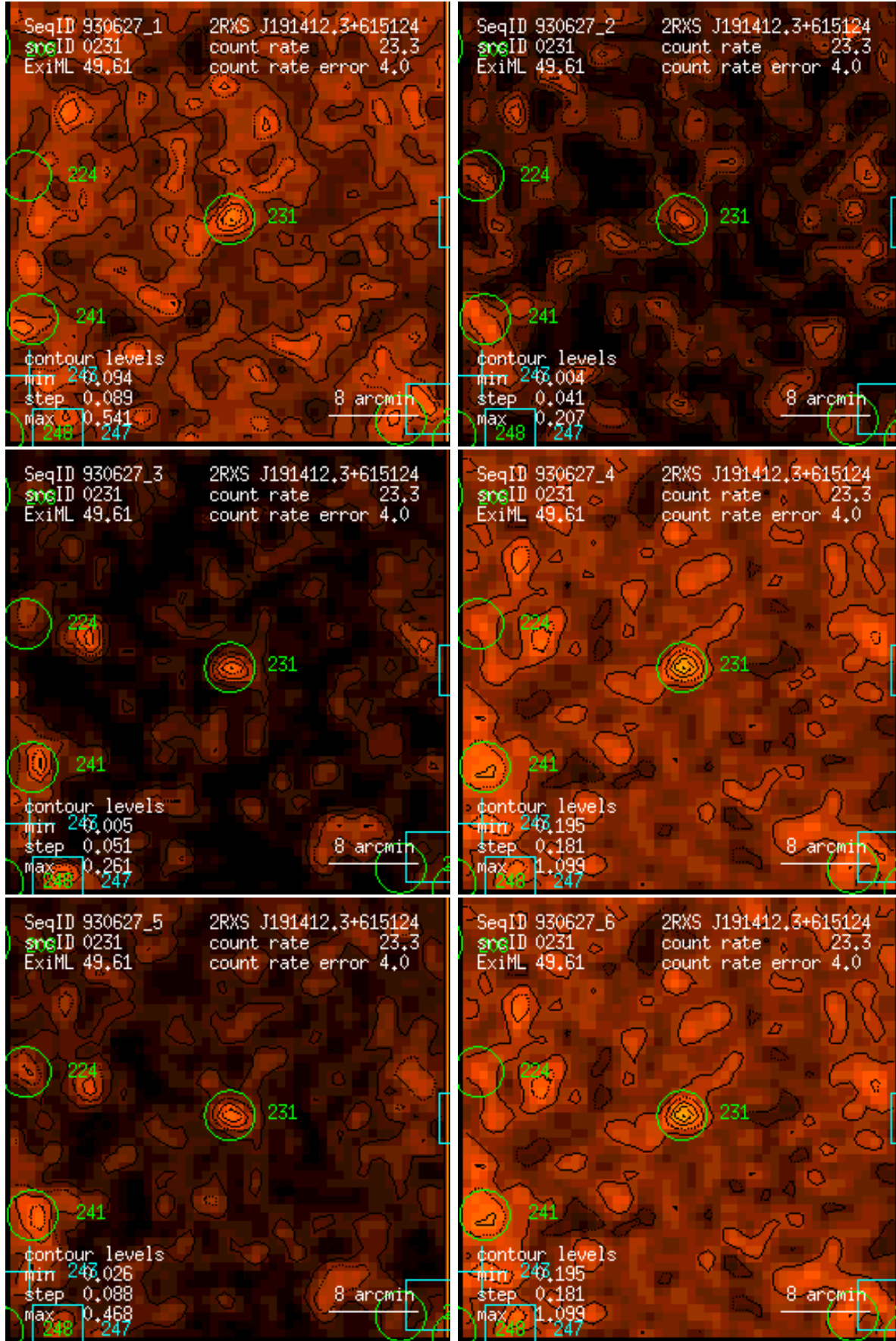
Figure 231: RASS 930627: detection 0231: band rate images, Gaussian filter: (1) PSPC channels 11 – 41, (2) 52 – 90, (3) 91 – 201, (4) 11 – 235, (5) 52 – 201, (6) 11 – 201. Broad band rates in counts/ks. Band rate contour levels in counts/ks/arcmin 2 .
