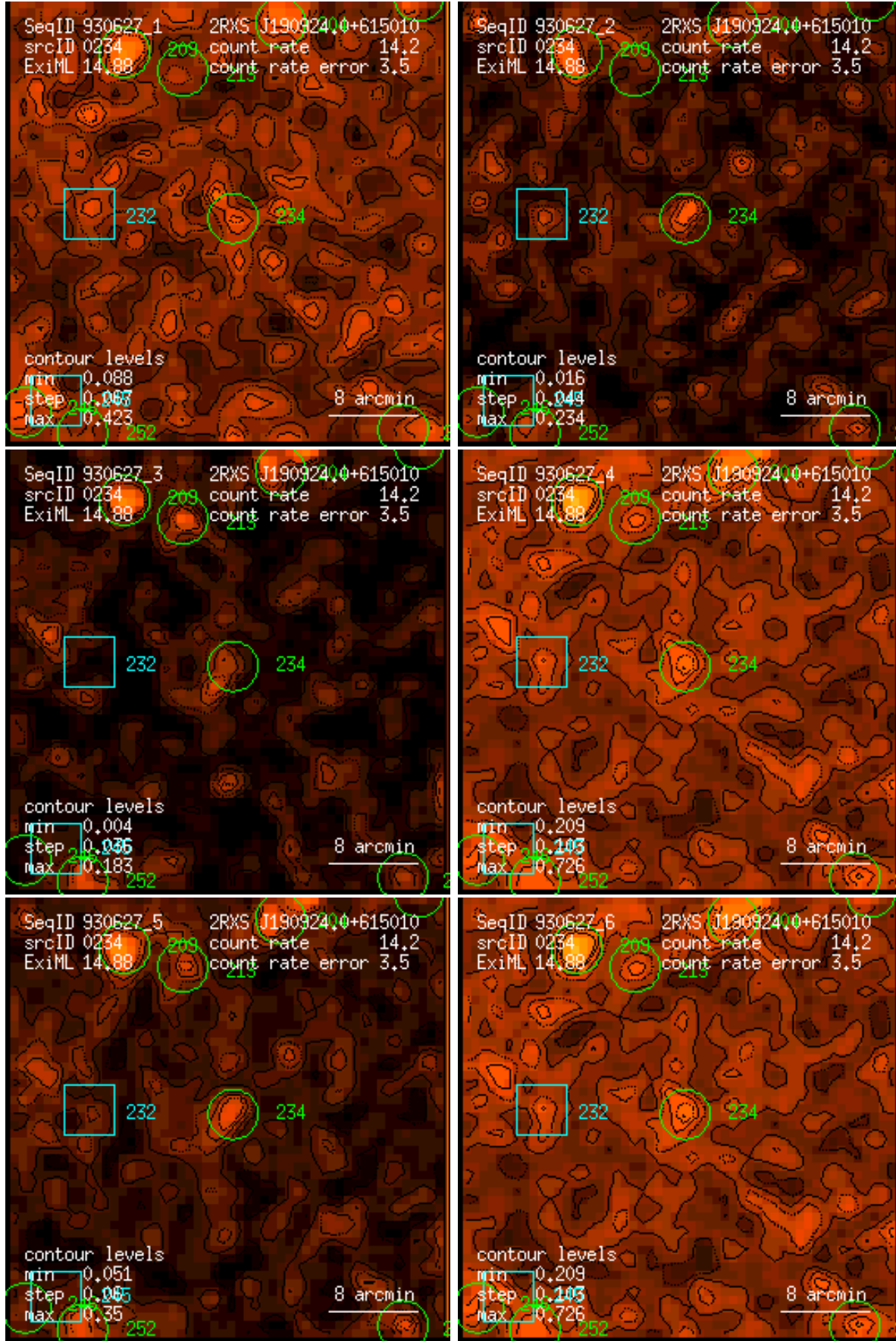
Figure 234: RASS 930627: detection 0234: band rate images, Gaussian filter: (1) PSPC channels 11 – 41, (2) 52 – 90, (3) 91 – 201, (4) 11 – 235, (5) 52 – 201, (6) 11 – 201. Broad band rates in counts/ks. Band rate contour levels in counts/ks/arcmin 2 .
