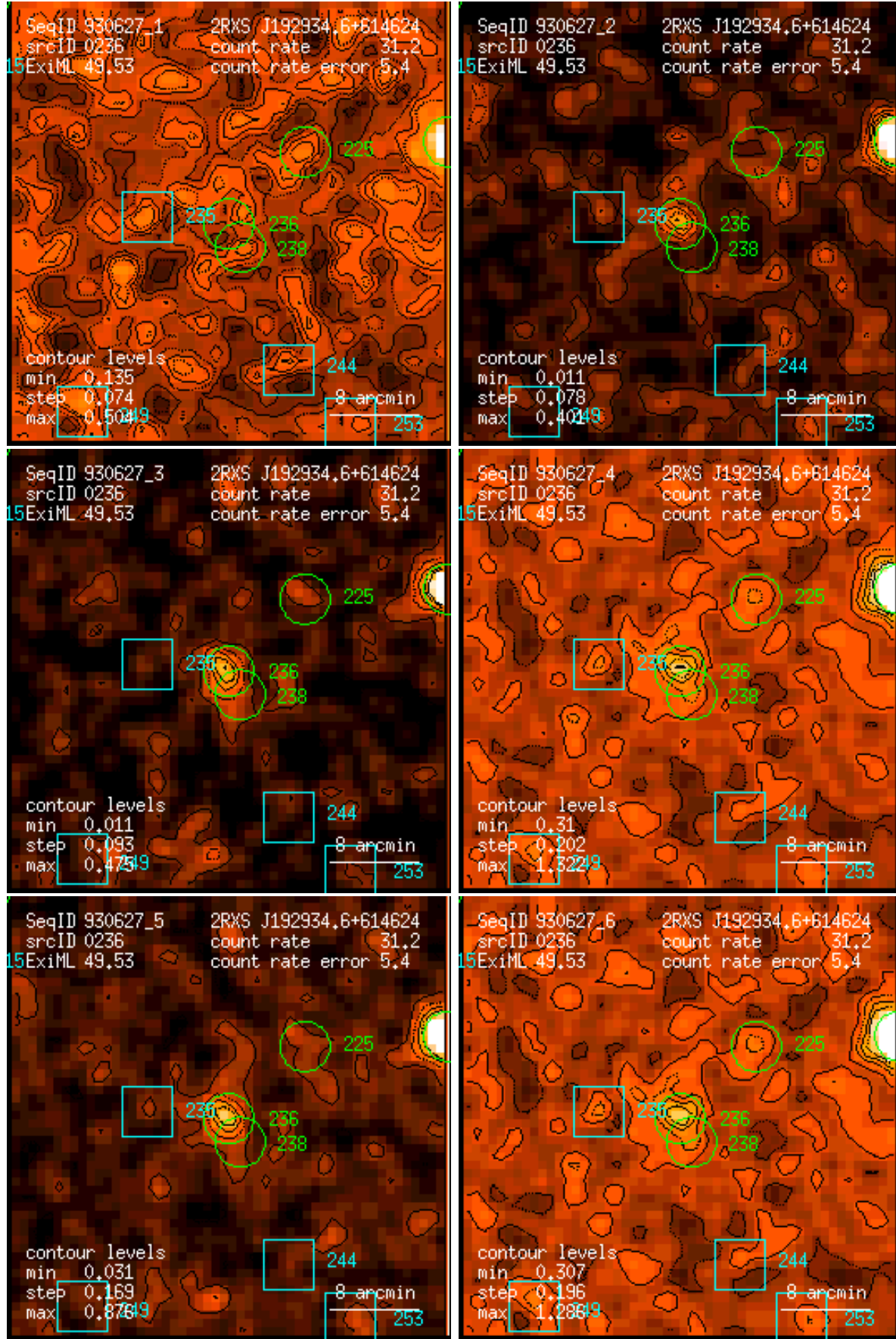
Figure 236: RASS 930627: detection 0236: band rate images, Gaussian filter: (1) PSPC channels 11 – 41, (2) 52 – 90, (3) 91 – 201, (4) 11 – 235, (5) 52 – 201, (6) 11 – 201. Broad band rates in counts/ks. Band rate contour levels in counts/ks/arcmin 2 .
