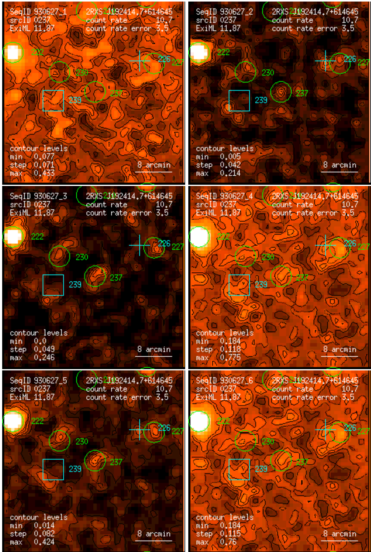
Figure 237: RASS 930627: detection 0237: band rate images, Gaussian filter: (1) PSPC channels 11 – 41, (2) 52 – 90, (3) 91 – 201, (4) 11 – 235, (5) 52 – 201, (6) 11 – 201. Broad band rates in counts/ks. Band rate contour levels in counts/ks/arcmin 2 .
