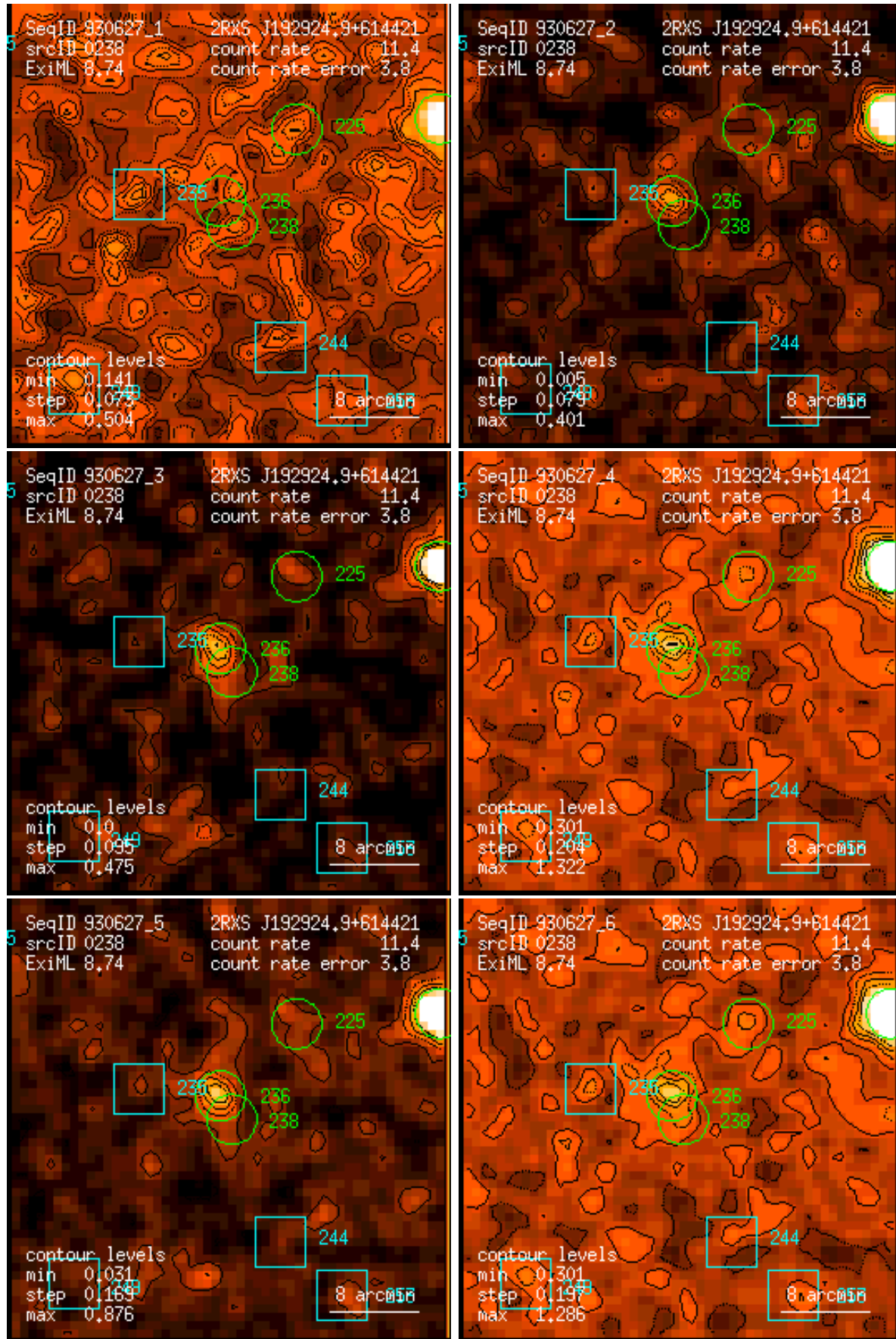
Figure 238: RASS 930627: detection 0238: band rate images, Gaussian filter: (1) PSPC channels 11 – 41, (2) 52 – 90, (3) 91 – 201, (4) 11 – 235, (5) 52 – 201, (6) 11 – 201. Broad band rates in counts/ks. Band rate contour levels in counts/ks/arcmin 2 .
