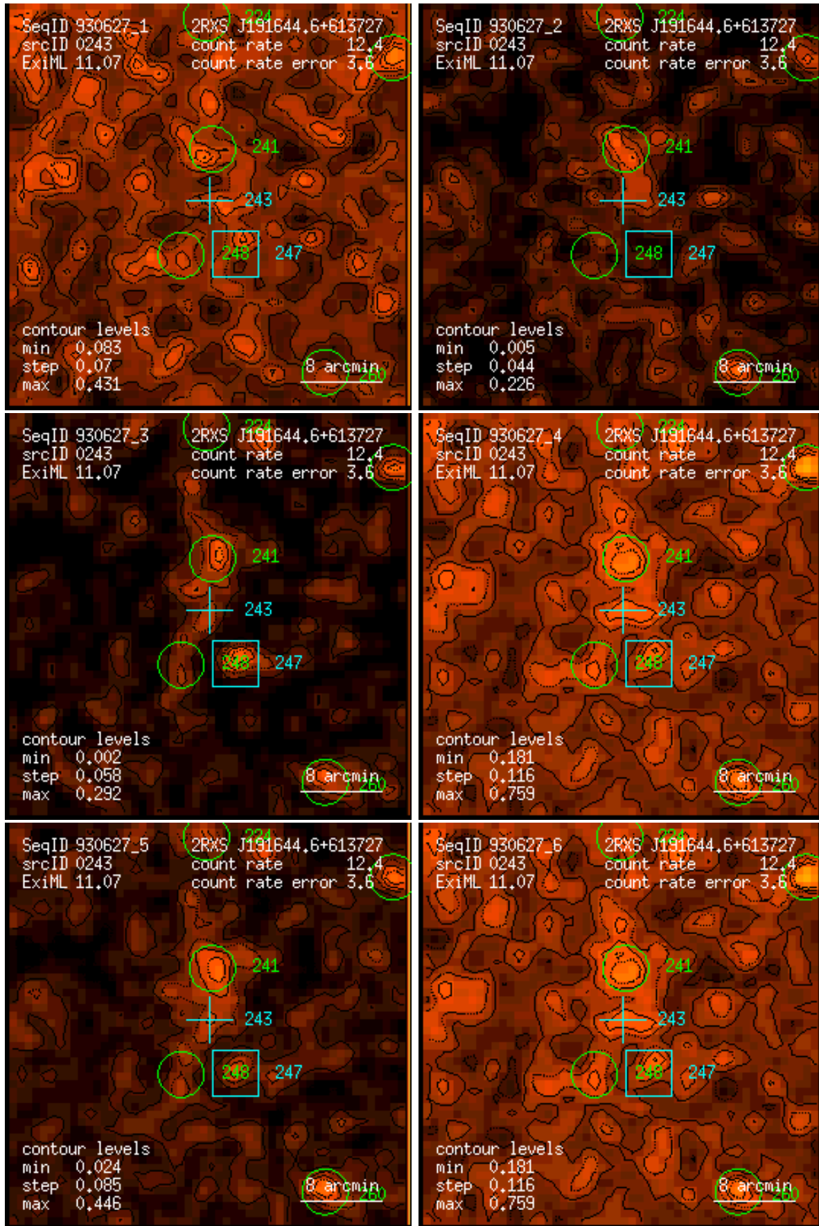
Figure 243: RASS 930627: detection 0243: band rate images, Gaussian filter: (1) PSPC channels 11 – 41, (2) 52 – 90, (3) 91 – 201, (4) 11 – 235, (5) 52 – 201, (6) 11 – 201. Broad band rates in counts/ks. Band rate contour levels in counts/ks/arcmin 2 .
