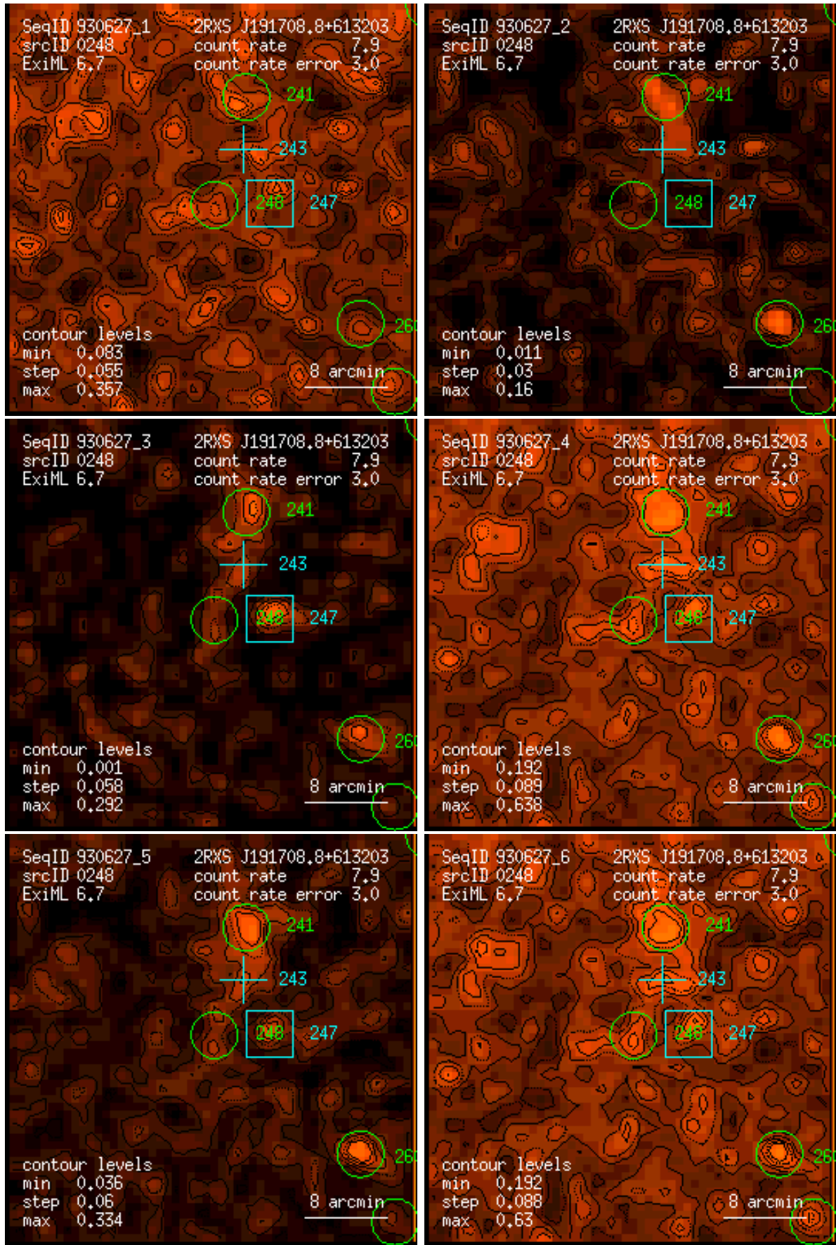
Figure 248: RASS 930627: detection 0248: band rate images, Gaussian filter: (1) PSPC channels 11 – 41, (2) 52 – 90, (3) 91 – 201, (4) 11 – 235, (5) 52 – 201, (6) 11 – 201. Broad band rates in counts/ks. Band rate contour levels in counts/ks/arcmin 2 .
