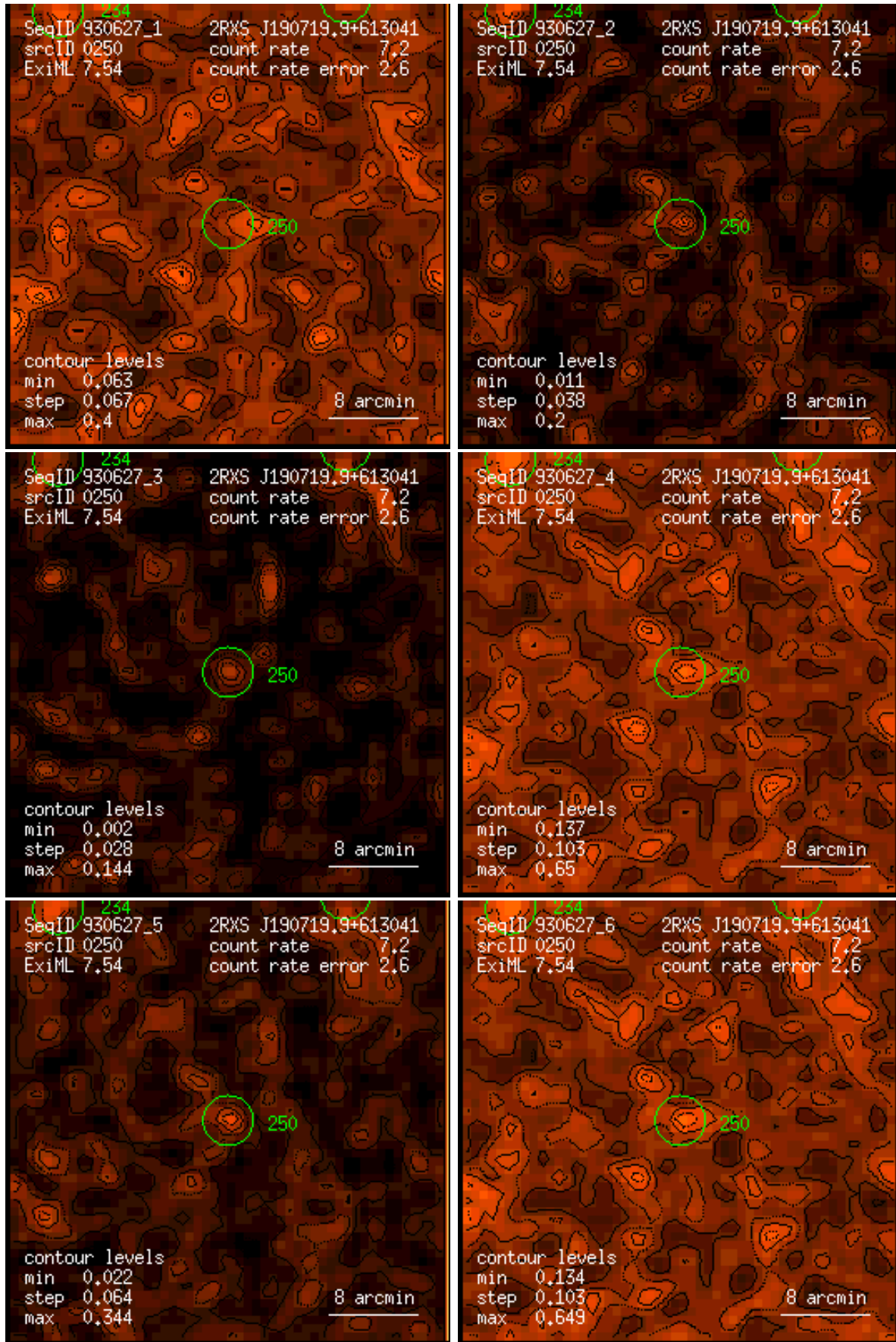
Figure 250: RASS 930627: detection 0250: band rate images, Gaussian filter: (1) PSPC channels 11 – 41, (2) 52 – 90, (3) 91 – 201, (4) 11 – 235, (5) 52 – 201, (6) 11 – 201. Broad band rates in counts/ks. Band rate contour levels in counts/ks/arcmin 2 .
