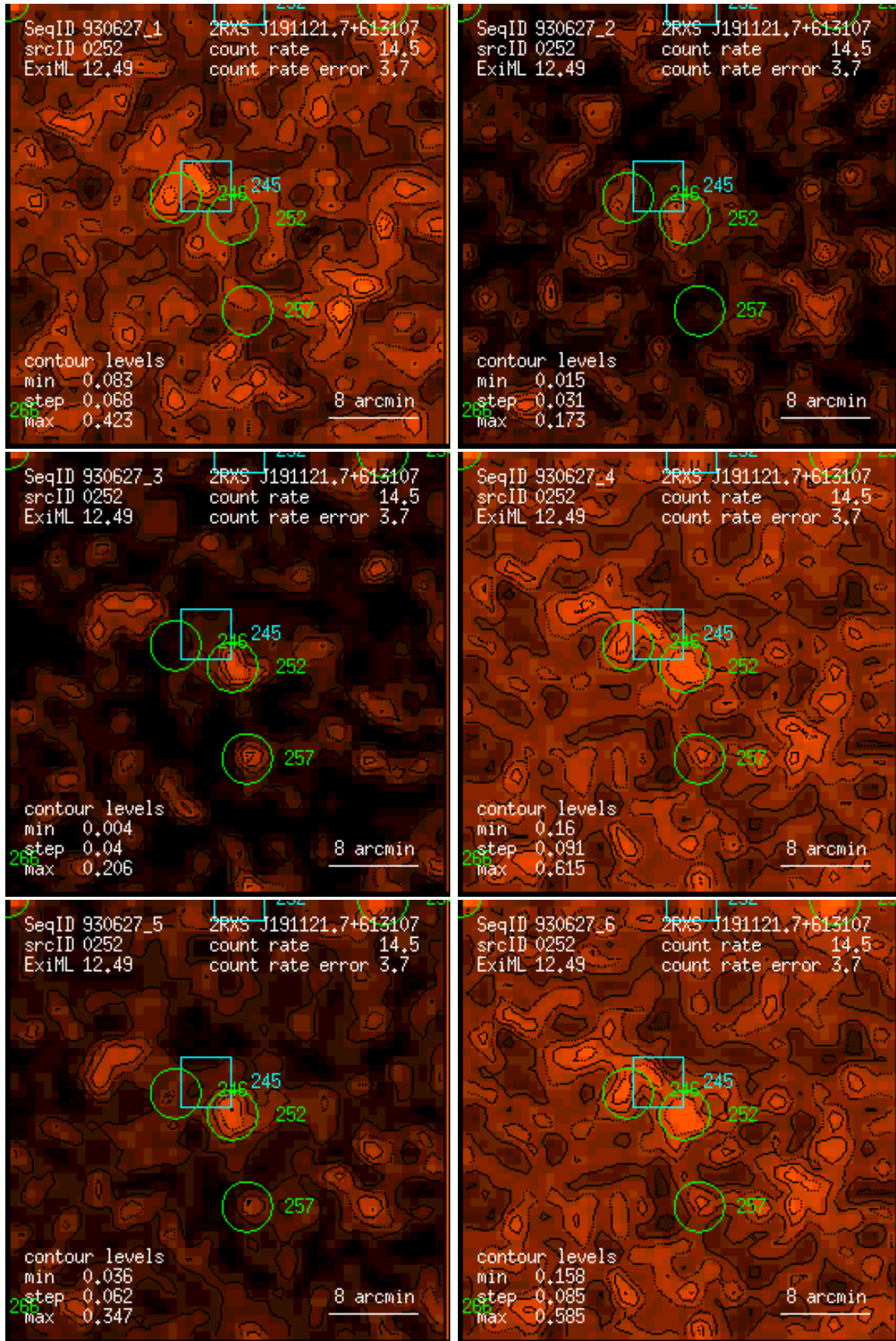
Figure 252: RASS 930627: detection 0252: band rate images, Gaussian filter: (1) PSPC channels 11 – 41, (2) 52 – 90, (3) 91 – 201, (4) 11 – 235, (5) 52 – 201, (6) 11 – 201. Broad band rates in counts/ks. Band rate contour levels in counts/ks/arcmin 2 .
