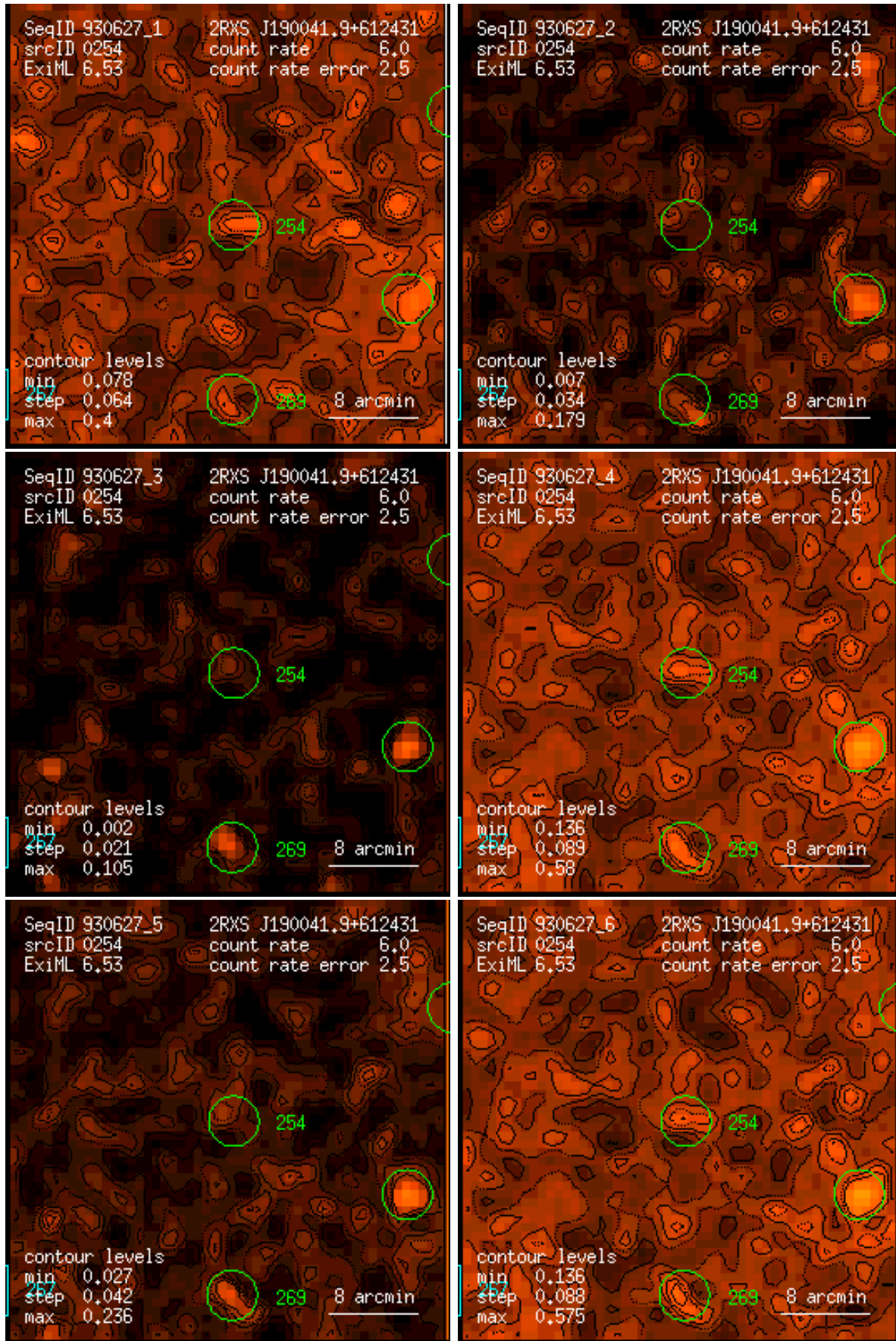
Figure 254: RASS 930627: detection 0254: band rate images, Gaussian filter: (1) PSPC channels 11 – 41, (2) 52 – 90, (3) 91 – 201, (4) 11 – 235, (5) 52 – 201, (6) 11 – 201. Broad band rates in counts/ks. Band rate contour levels in counts/ks/arcmin 2 .
