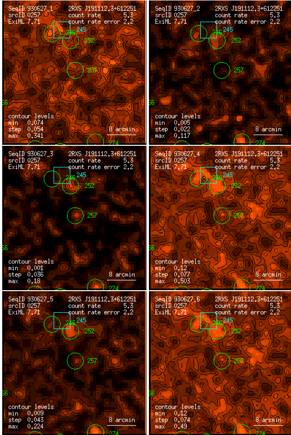
Figure 257: RASS 930627: detection 0257: band rate images, Gaussian filter: (1) PSPC channels 11 – 41, (2) 52 – 90, (3) 91 – 201, (4) 11 – 235, (5) 52 – 201, (6) 11 – 201. Broad band rates in counts/ks. Band rate contour levels in counts/ks/arcmin 2 .
