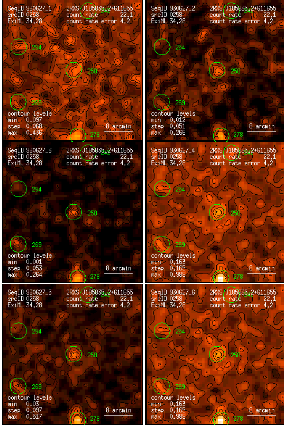
Figure 258: RASS 930627: detection 0258: band rate images, Gaussian filter: (1) PSPC channels 11 – 41, (2) 52 – 90, (3) 91 – 201, (4) 11 – 235, (5) 52 – 201, (6) 11 – 201. Broad band rates in counts/ks. Band rate contour levels in counts/ks/arcmin 2 .
